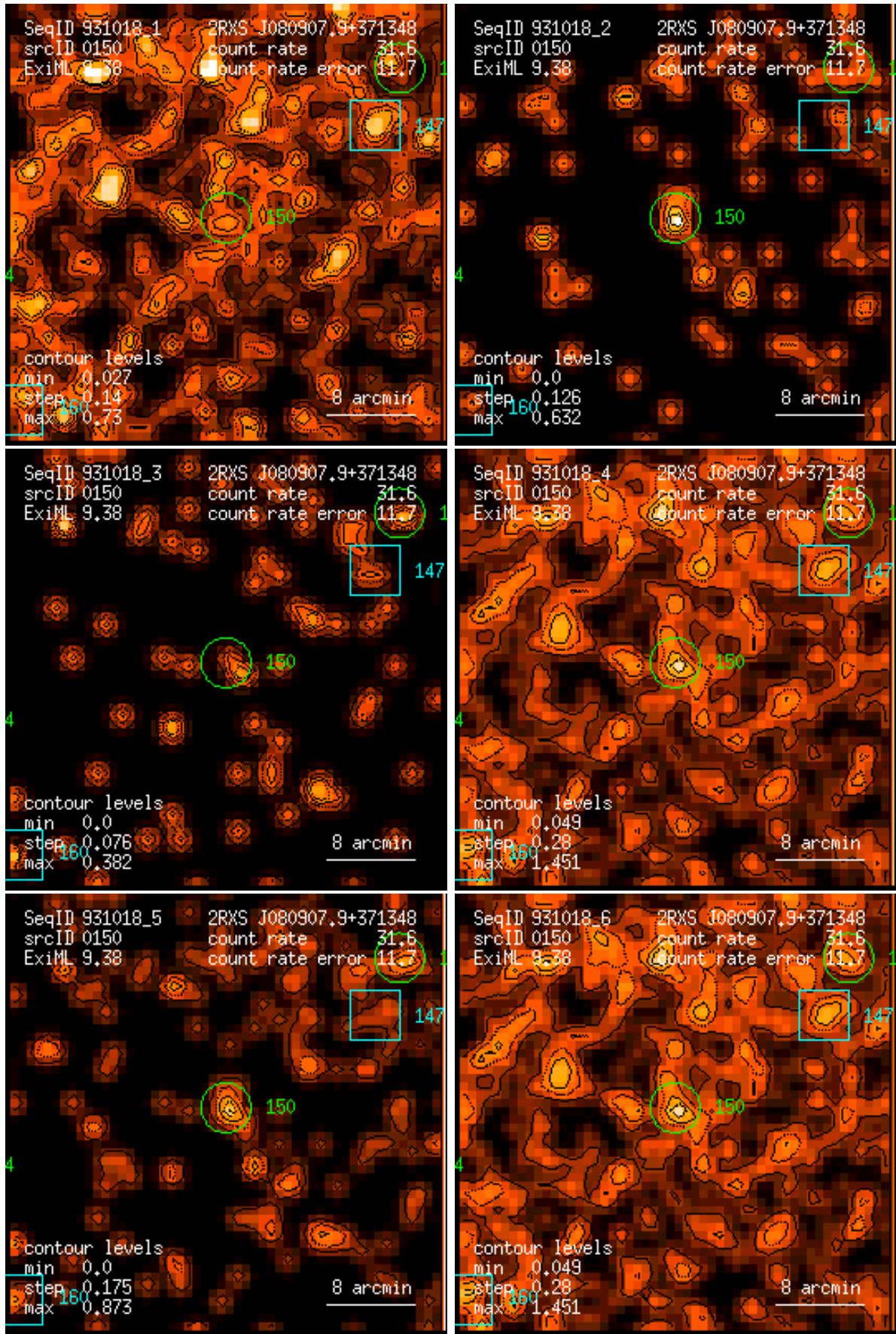
Figure 150: RASS 931018: detection 0150: band rate images, Gaussian filter: (1) PSPC channels 11 – 41, (2) 52 – 90, (3) 91 – 201, (4) 11 – 235, (5) 52 – 201, (6) 11 – 201. Broad band rates in counts/ks. Band rate contour levels in counts/ks/arcmin 2 .
