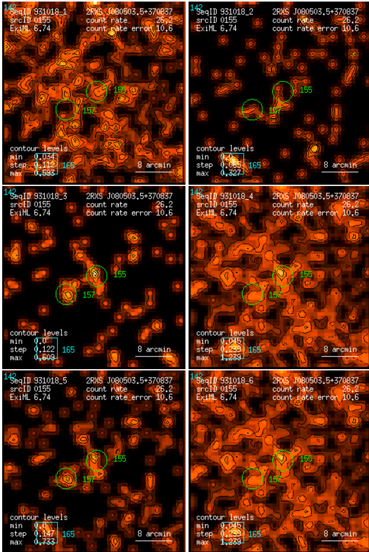
Figure 155: RASS 931018: detection 0155: band rate images, Gaussian filter: (1) PSPC channels 11 – 41, (2) 52 – 90, (3) 91 – 201, (4) 11 – 235, (5) 52 – 201, (6) 11 – 201. Broad band rates in counts/ks. Band rate contour levels in counts/ks/arcmin 2 .
