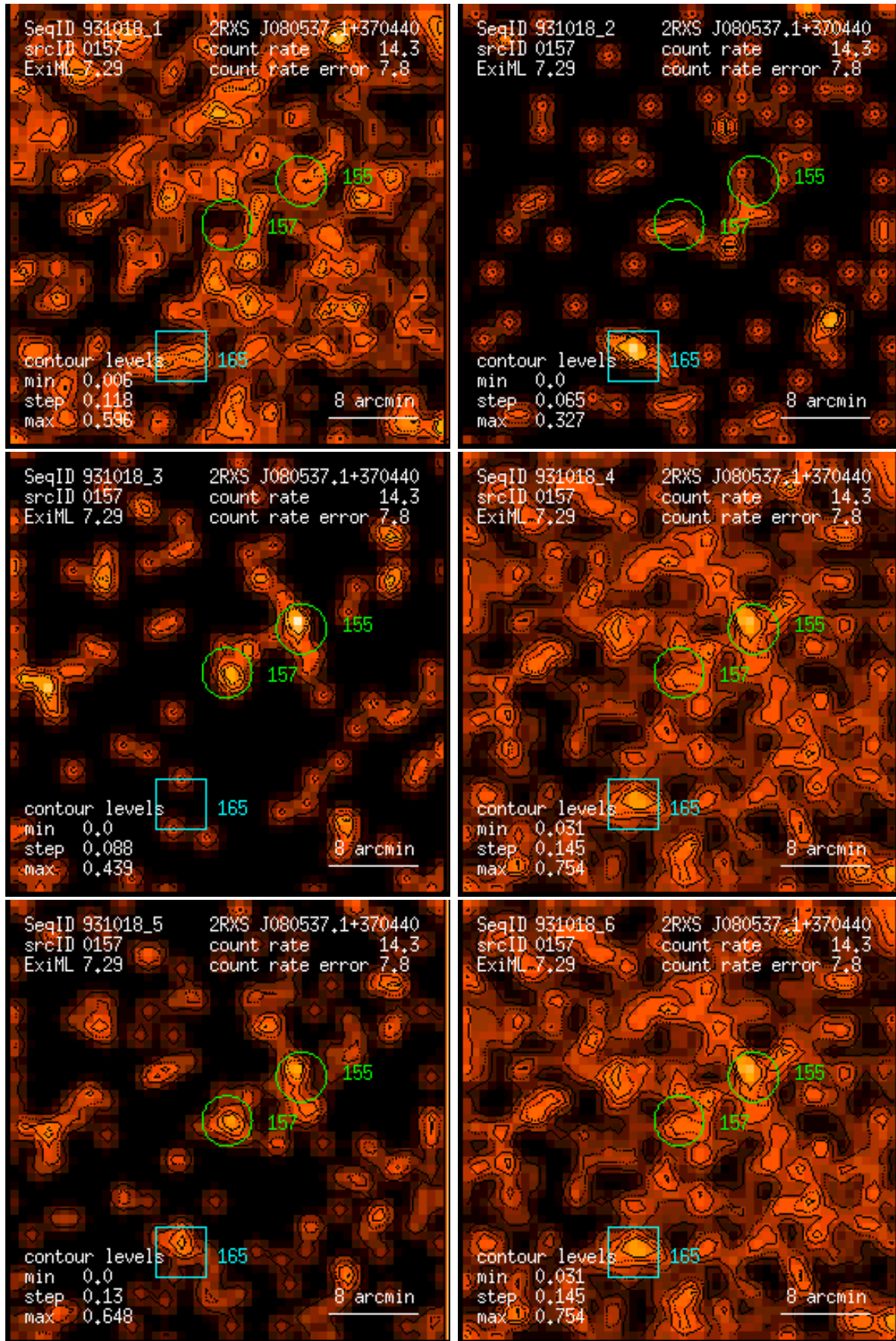
Figure 157: RASS 931018: detection 0157: band rate images, Gaussian filter: (1) PSPC channels 11 – 41, (2) 52 – 90, (3) 91 – 201, (4) 11 – 235, (5) 52 – 201, (6) 11 – 201. Broad band rates in counts/ks. Band rate contour levels in counts/ks/arcmin 2 .
