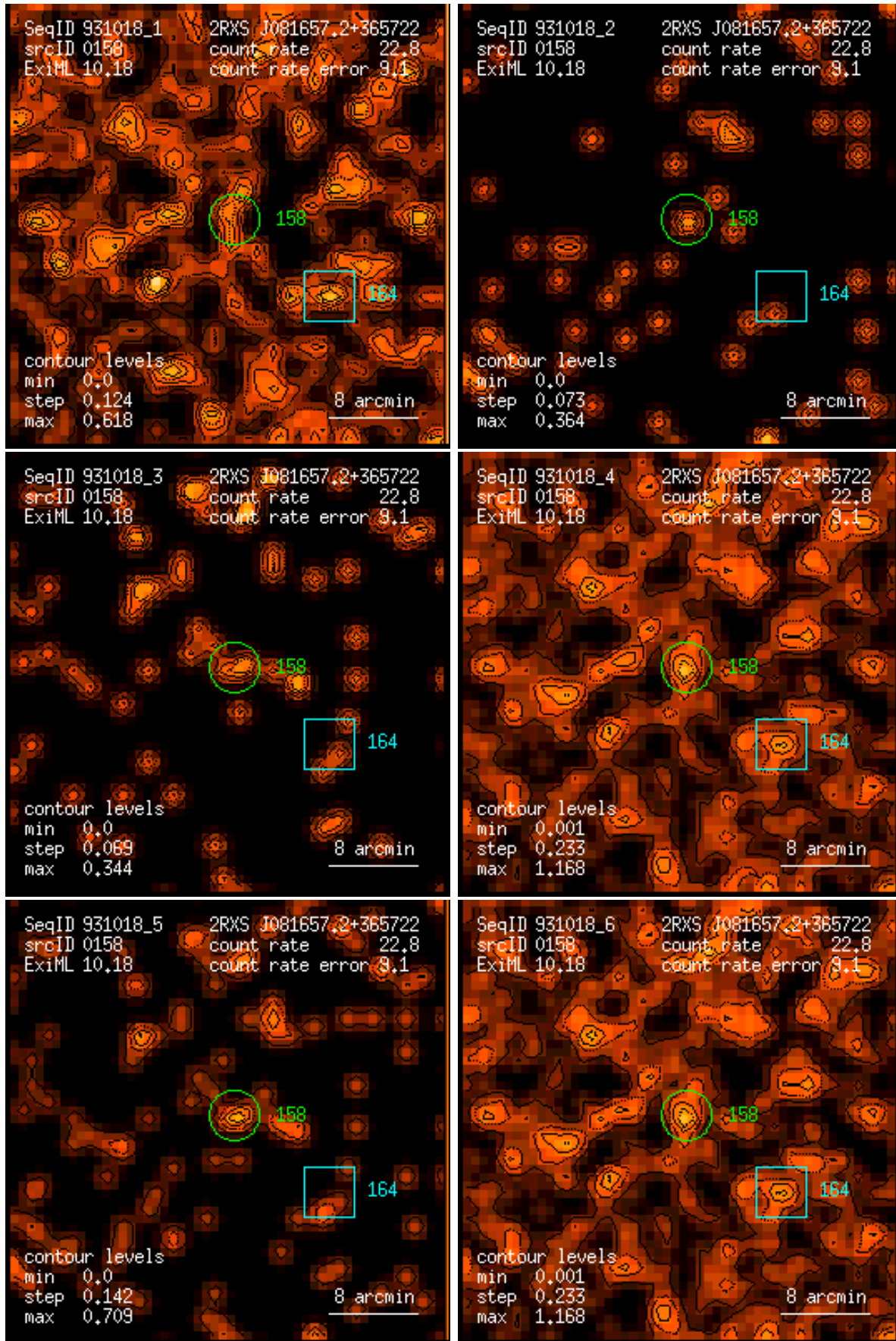
Figure 158: RASS 931018: detection 0158: band rate images, Gaussian filter: (1) PSPC channels 11 – 41, (2) 52 – 90, (3) 91 – 201, (4) 11 – 235, (5) 52 – 201, (6) 11 – 201. Broad band rates in counts/ks. Band rate contour levels in counts/ks/arcmin 2 .
