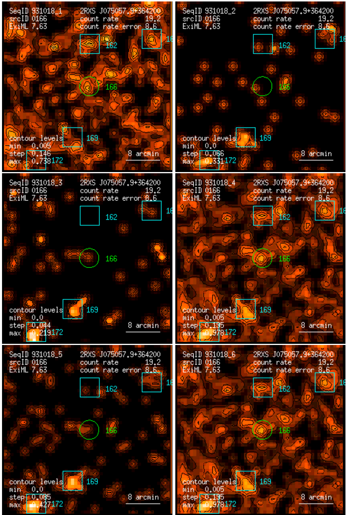
Figure 166: RASS 931018: detection 0166: band rate images, Gaussian filter: (1) PSPC channels 11 – 41, (2) 52 – 90, (3) 91 – 201, (4) 11 – 235, (5) 52 – 201, (6) 11 – 201. Broad band rates in counts/ks. Band rate contour levels in counts/ks/arcmin 2 .
