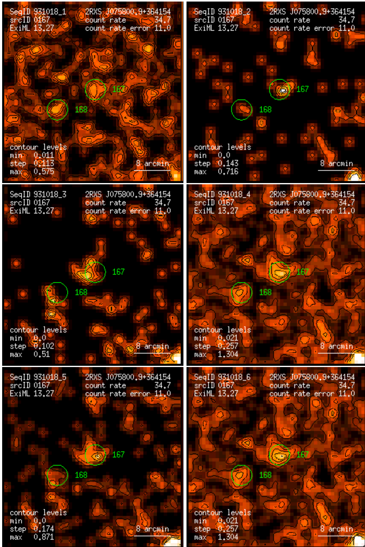
Figure 167: RASS 931018: detection 0167: band rate images, Gaussian filter: (1) PSPC channels 11 – 41, (2) 52 – 90, (3) 91 – 201, (4) 11 – 235, (5) 52 – 201, (6) 11 – 201. Broad band rates in counts/ks. Band rate contour levels in counts/ks/arcmin 2 .
