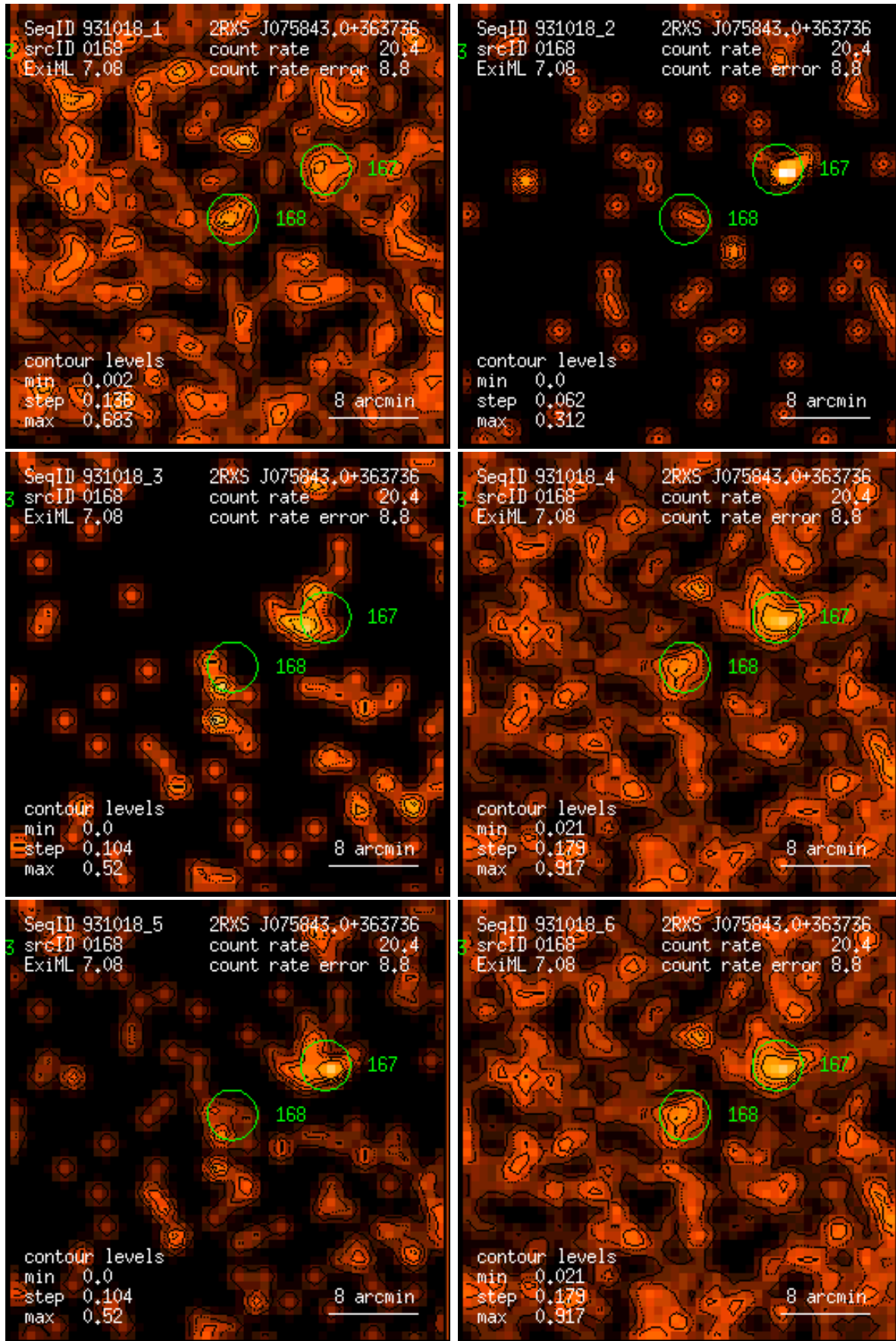
Figure 168: RASS 931018: detection 0168: band rate images, Gaussian filter: (1) PSPC channels 11 – 41, (2) 52 – 90, (3) 91 – 201, (4) 11 – 235, (5) 52 – 201, (6) 11 – 201. Broad band rates in counts/ks. Band rate contour levels in counts/ks/arcmin 2 .
