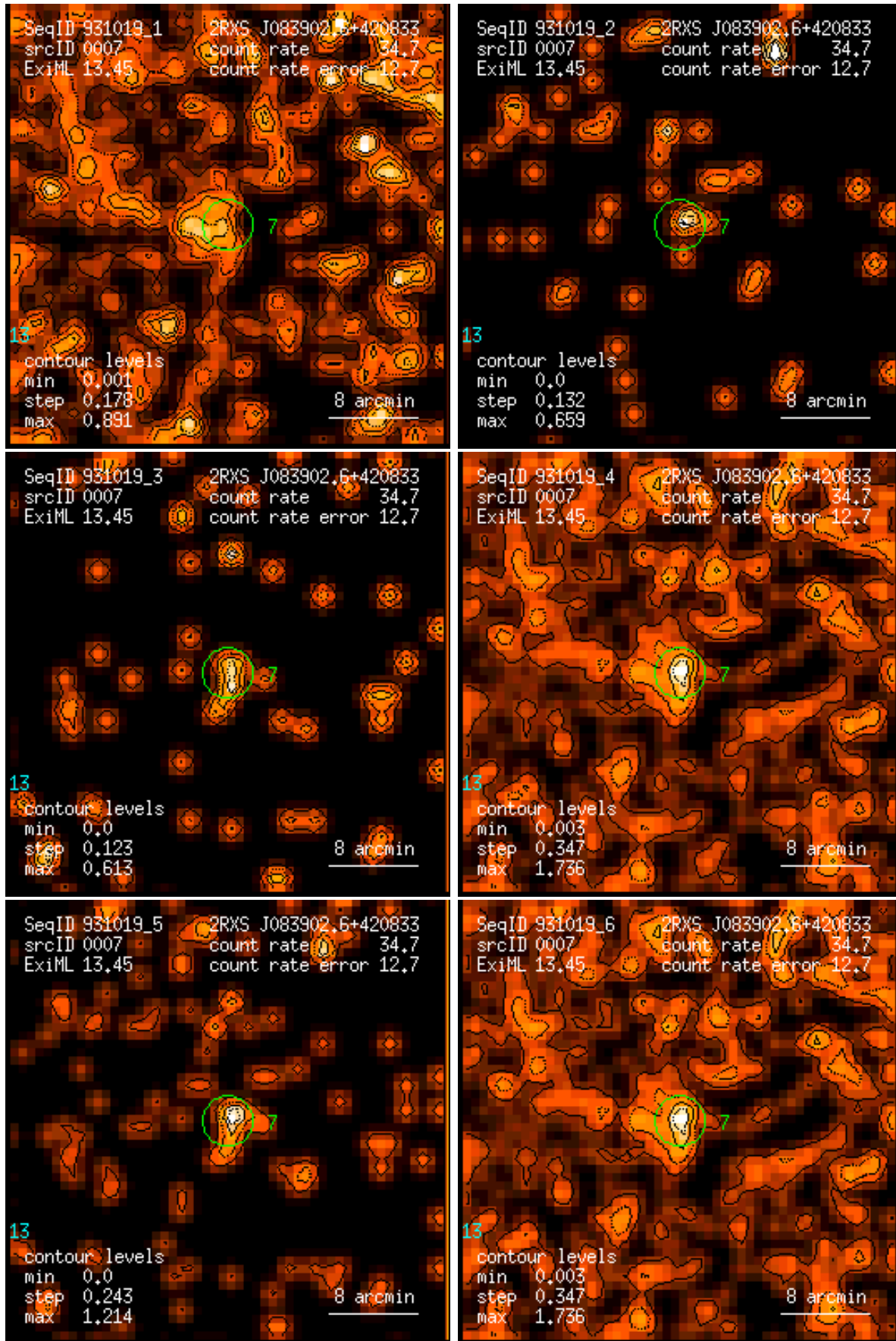
Figure 7: RASS 931019: detection 0007: band rate images, Gaussian filter: (1) PSPC channels 11 – 41, (2) 52 – 90, (3) 91 – 201, (4) 11 – 235, (5) 52 – 201, (6) 11 – 201. Broad band rates in counts/ks. Band rate contour levels in counts/ks/arcmin 2 .
