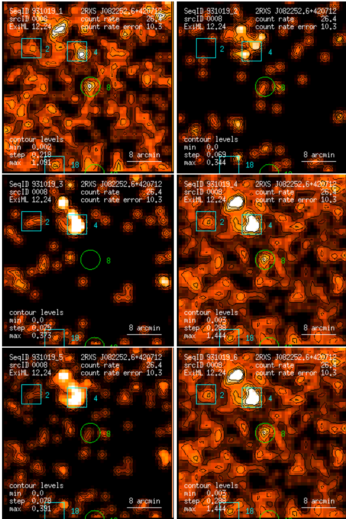
Figure 8: RASS 931019: detection 0008: band rate images, Gaussian filter: (1) PSPC channels 11 – 41, (2) 52 – 90, (3) 91 – 201, (4) 11 – 235, (5) 52 – 201, (6) 11 – 201. Broad band rates in counts/ks. Band rate contour levels in counts/ks/arcmin 2 .
