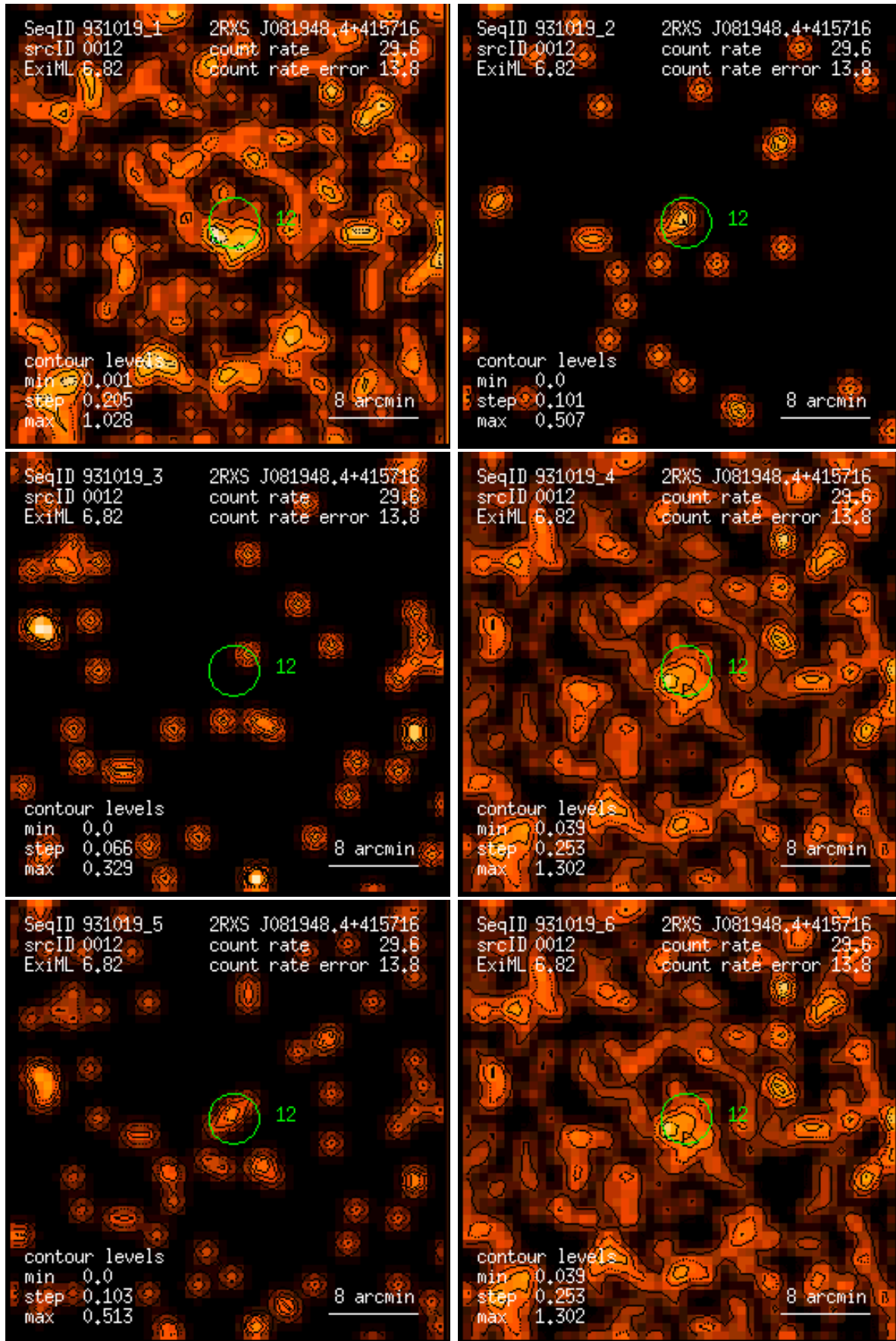
Figure 12: RASS 931019: detection 0012: band rate images, Gaussian filter: (1) PSPC channels 11 – 41, (2) 52 – 90, (3) 91 – 201, (4) 11 – 235, (5) 52 – 201, (6) 11 – 201. Broad band rates in counts/ks. Band rate contour levels in counts/ks/arcmin 2 .
