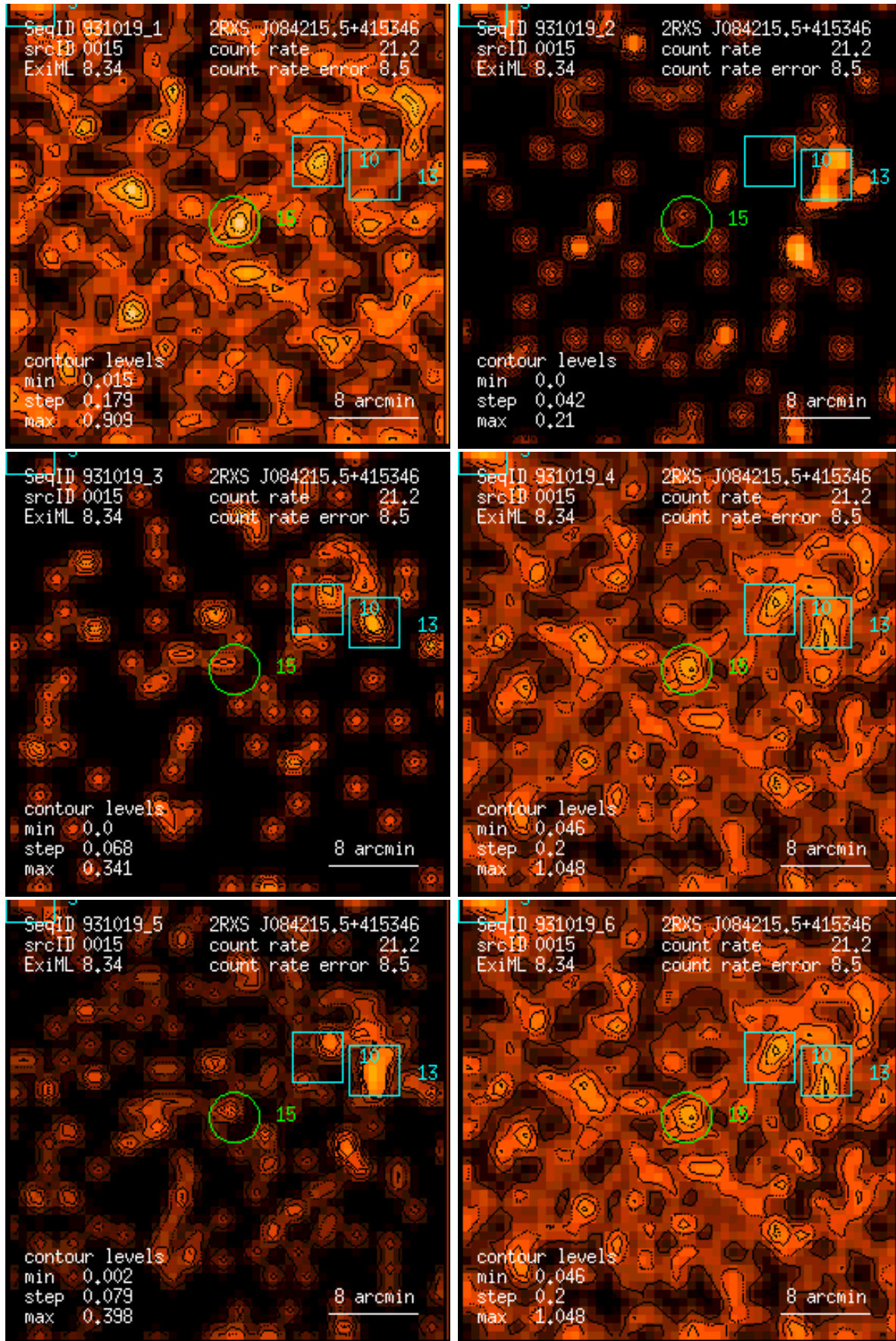
Figure 15: RASS 931019: detection 0015: band rate images, Gaussian filter: (1) PSPC channels 11 – 41, (2) 52 – 90, (3) 91 – 201, (4) 11 – 235, (5) 52 – 201, (6) 11 – 201. Broad band rates in counts/ks. Band rate contour levels in counts/ks/arcmin 2 .
