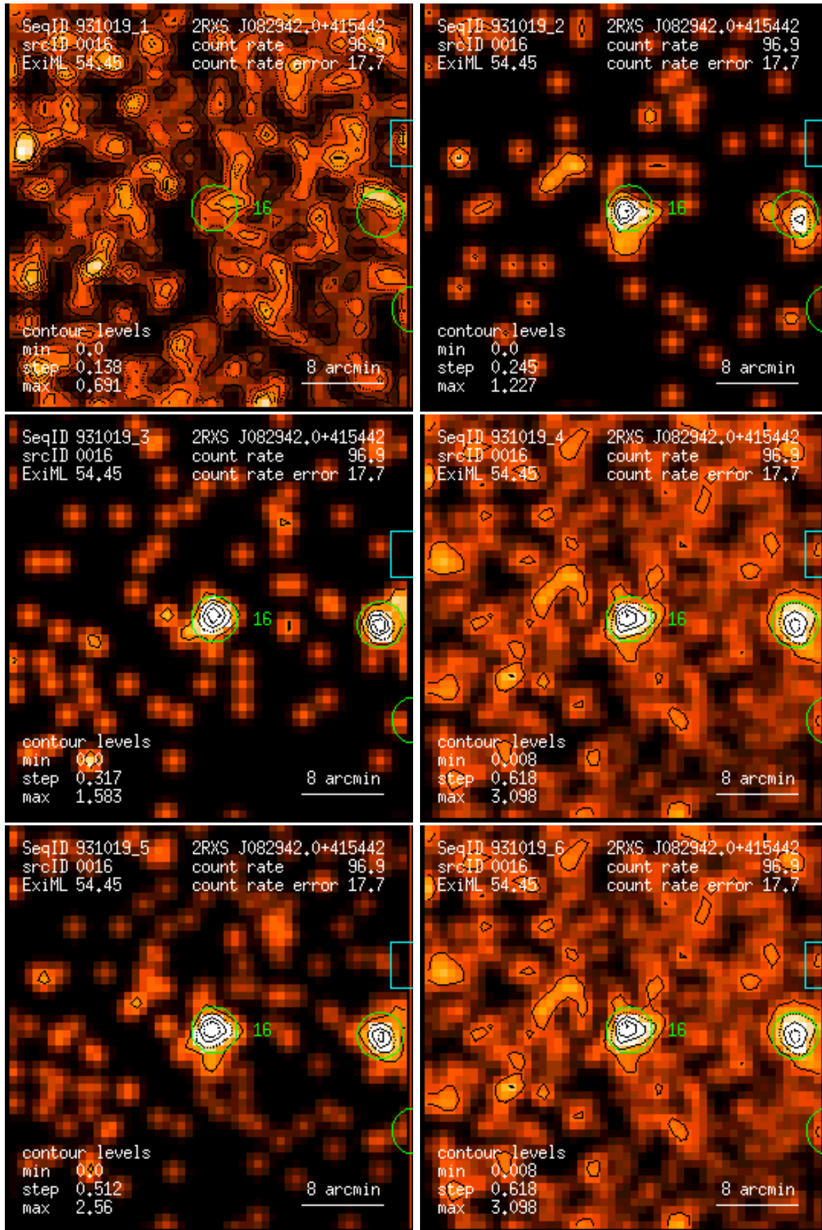
Figure 16: RASS 931019: detection 0016: band rate images, Gaussian filter: (1) PSPC channels 11 – 41, (2) 52 – 90, (3) 91 – 201, (4) 11 – 235, (5) 52 – 201, (6) 11 – 201. Broad band rates in counts/ks. Band rate contour levels in counts/ks/arcmin 2 .
