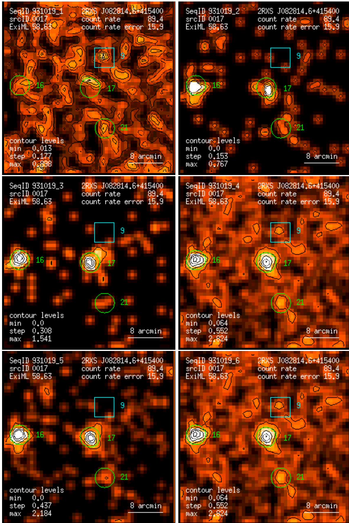
Figure 17: RASS 931019: detection 0017: band rate images, Gaussian filter: (1) PSPC channels 11 – 41, (2) 52 – 90, (3) 91 – 201, (4) 11 – 235, (5) 52 – 201, (6) 11 – 201. Broad band rates in counts/ks. Band rate contour levels in counts/ks/arcmin 2 .
