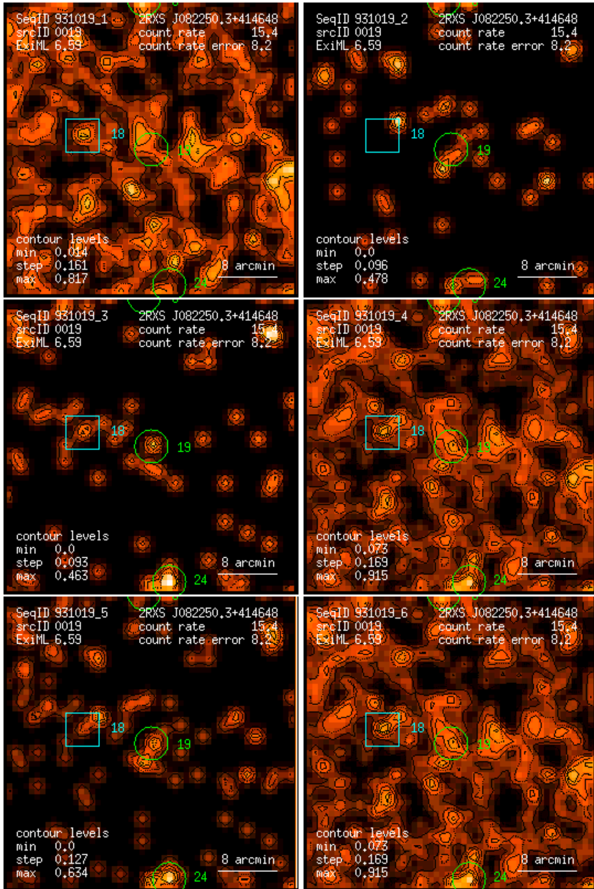
Figure 19: RASS 931019: detection 0019: band rate images, Gaussian filter: (1) PSPC channels 11 – 41, (2) 52 – 90, (3) 91 – 201, (4) 11 – 235, (5) 52 – 201, (6) 11 – 201. Broad band rates in counts/ks. Band rate contour levels in counts/ks/arcmin 2 .
