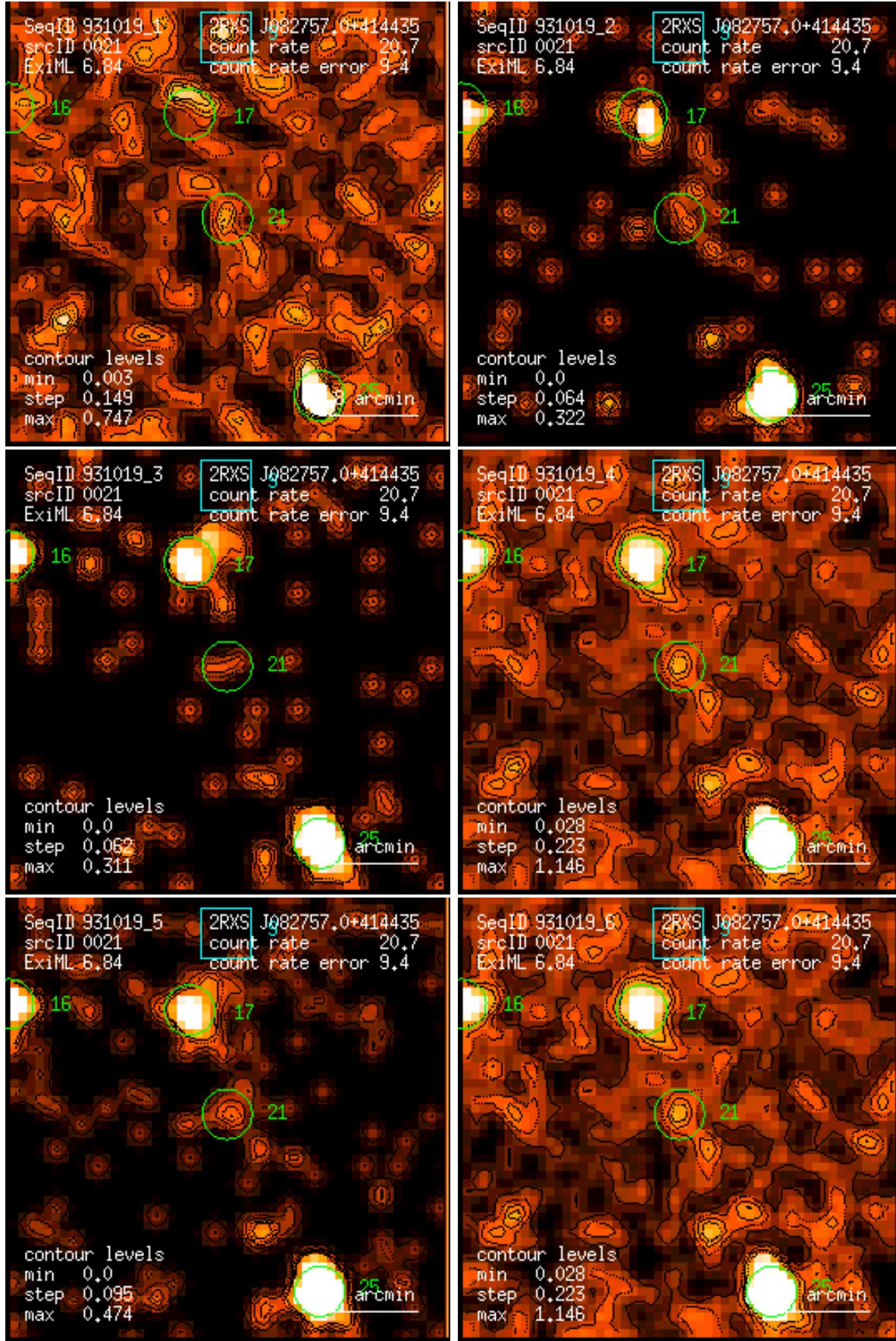
Figure 21: RASS 931019: detection 0021: band rate images, Gaussian filter: (1) PSPC channels 11 – 41, (2) 52 – 90, (3) 91 – 201, (4) 11 – 235, (5) 52 – 201, (6) 11 – 201. Broad band rates in counts/ks. Band rate contour levels in counts/ks/arcmin 2 .
