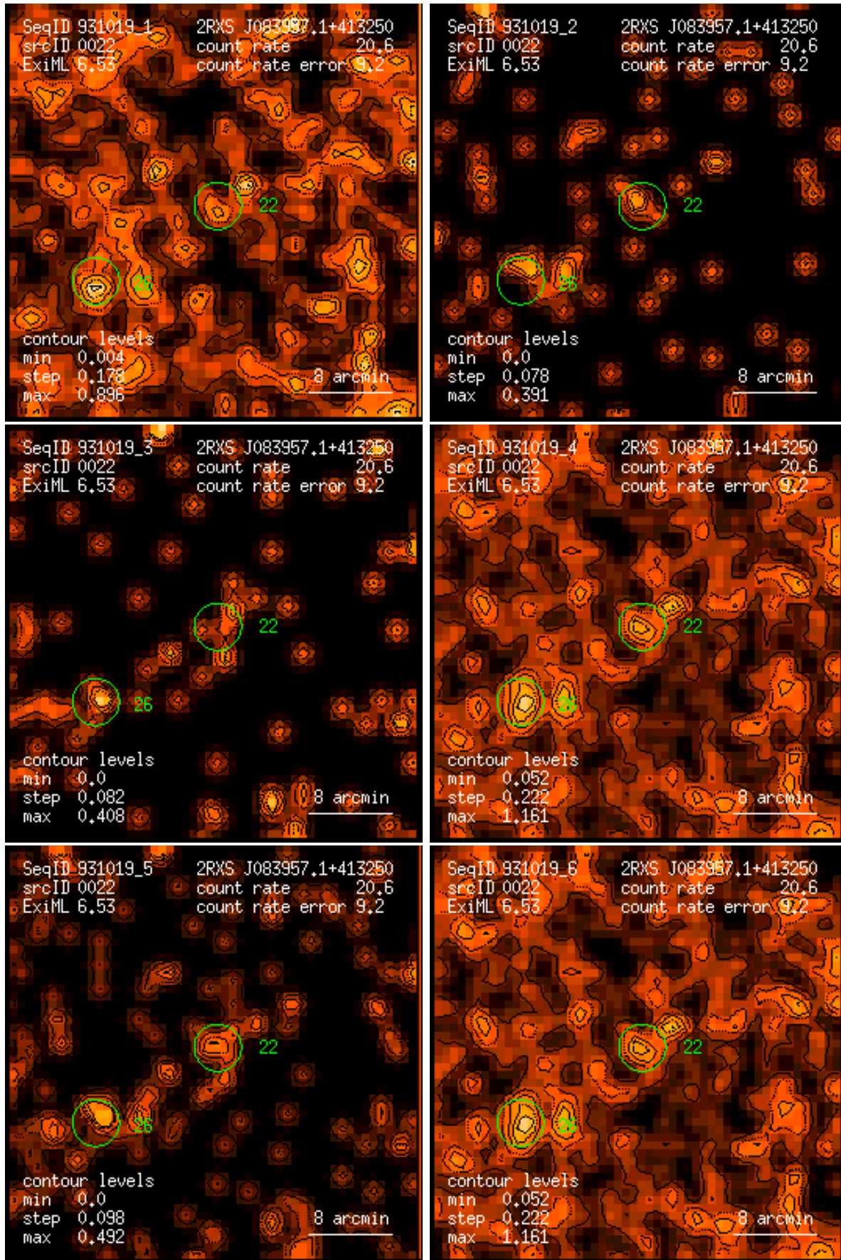
Figure 22: RASS 931019: detection 0022: band rate images, Gaussian filter: (1) PSPC channels 11 – 41, (2) 52 – 90, (3) 91 – 201, (4) 11 – 235, (5) 52 – 201, (6) 11 – 201. Broad band rates in counts/ks. Band rate contour levels in counts/ks/arcmin 2 .
