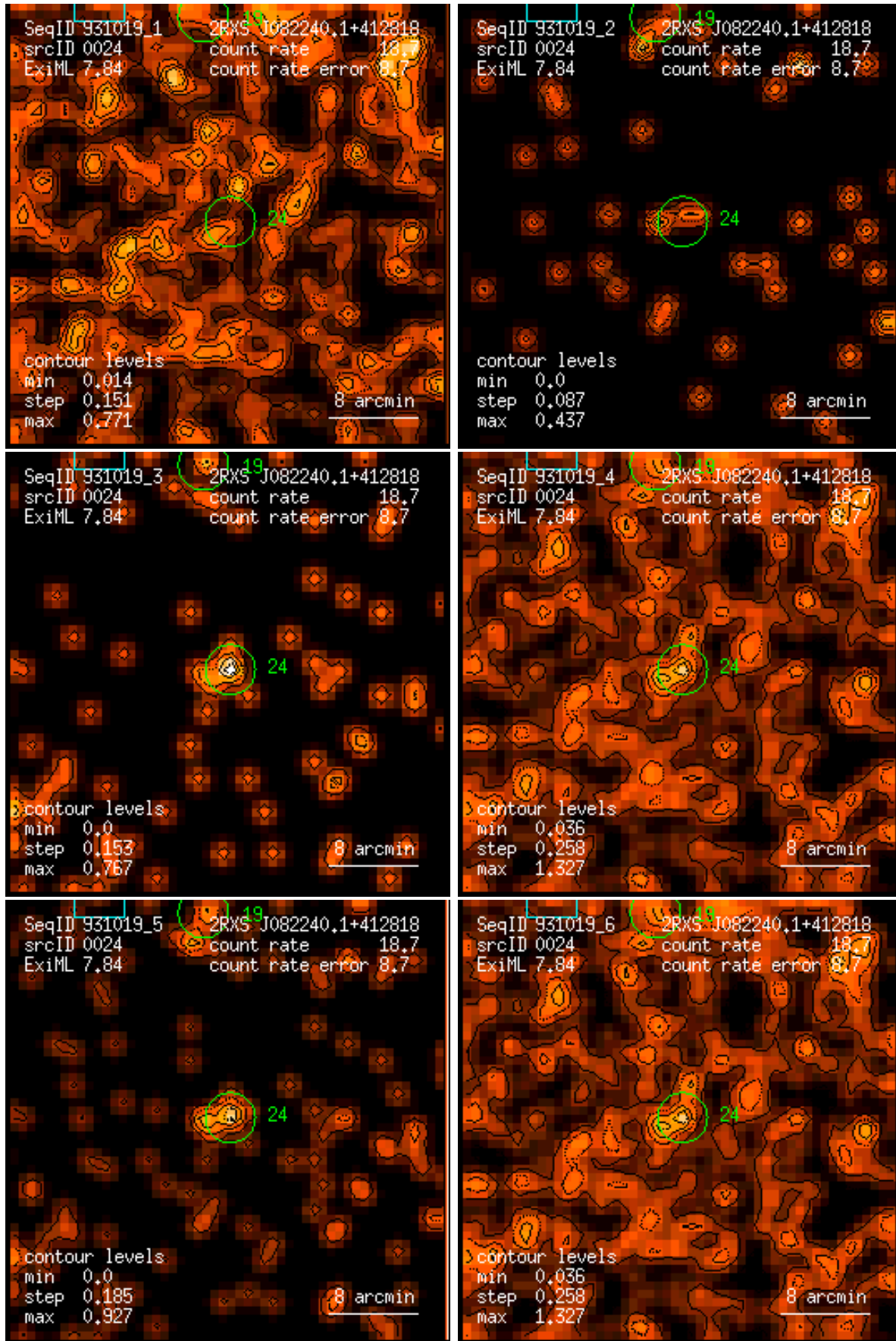
Figure 24: RASS 931019: detection 0024: band rate images, Gaussian filter: (1) PSPC channels 11 – 41, (2) 52 – 90, (3) 91 – 201, (4) 11 – 235, (5) 52 – 201, (6) 11 – 201. Broad band rates in counts/ks. Band rate contour levels in counts/ks/arcmin 2 .
