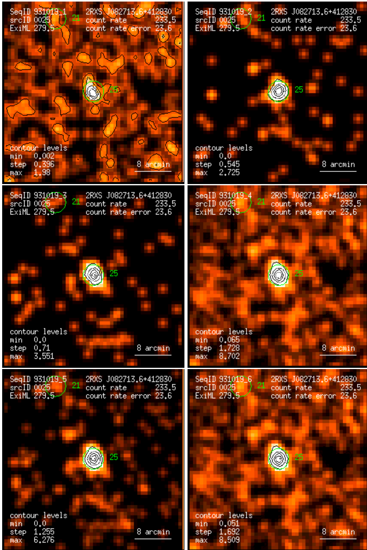
Figure 25: RASS 931019: detection 0025: band rate images, Gaussian filter: (1) PSPC channels 11 – 41, (2) 52 – 90, (3) 91 – 201, (4) 11 – 235, (5) 52 – 201, (6) 11 – 201. Broad band rates in counts/ks. Band rate contour levels in counts/ks/arcmin 2 .
