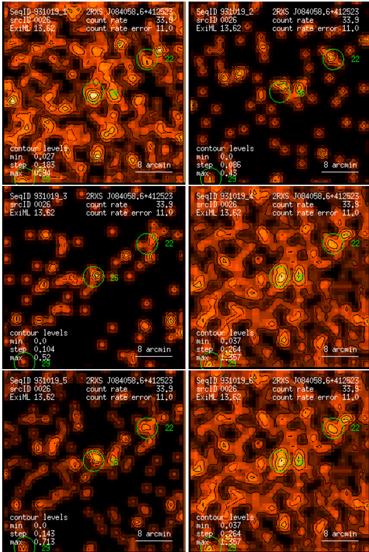
Figure 26: RASS 931019: detection 0026: band rate images, Gaussian filter: (1) PSPC channels 11 – 41, (2) 52 – 90, (3) 91 – 201, (4) 11 – 235, (5) 52 – 201, (6) 11 – 201. Broad band rates in counts/ks. Band rate contour levels in counts/ks/arcmin 2 .
