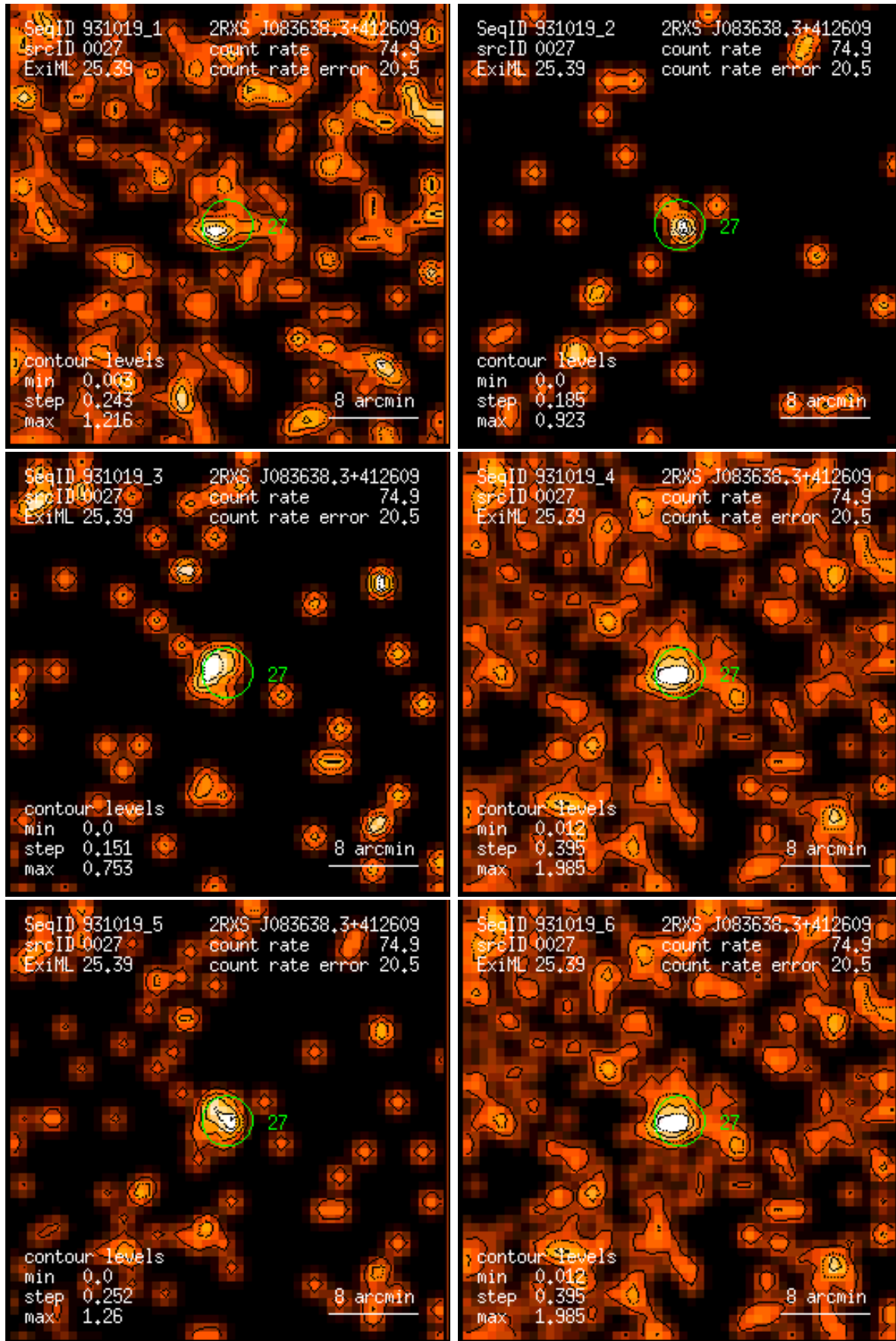
Figure 27: RASS 931019: detection 0027: band rate images, Gaussian filter: (1) PSPC channels 11 – 41, (2) 52 – 90, (3) 91 – 201, (4) 11 – 235, (5) 52 – 201, (6) 11 – 201. Broad band rates in counts/ks. Band rate contour levels in counts/ks/arcmin 2 .
