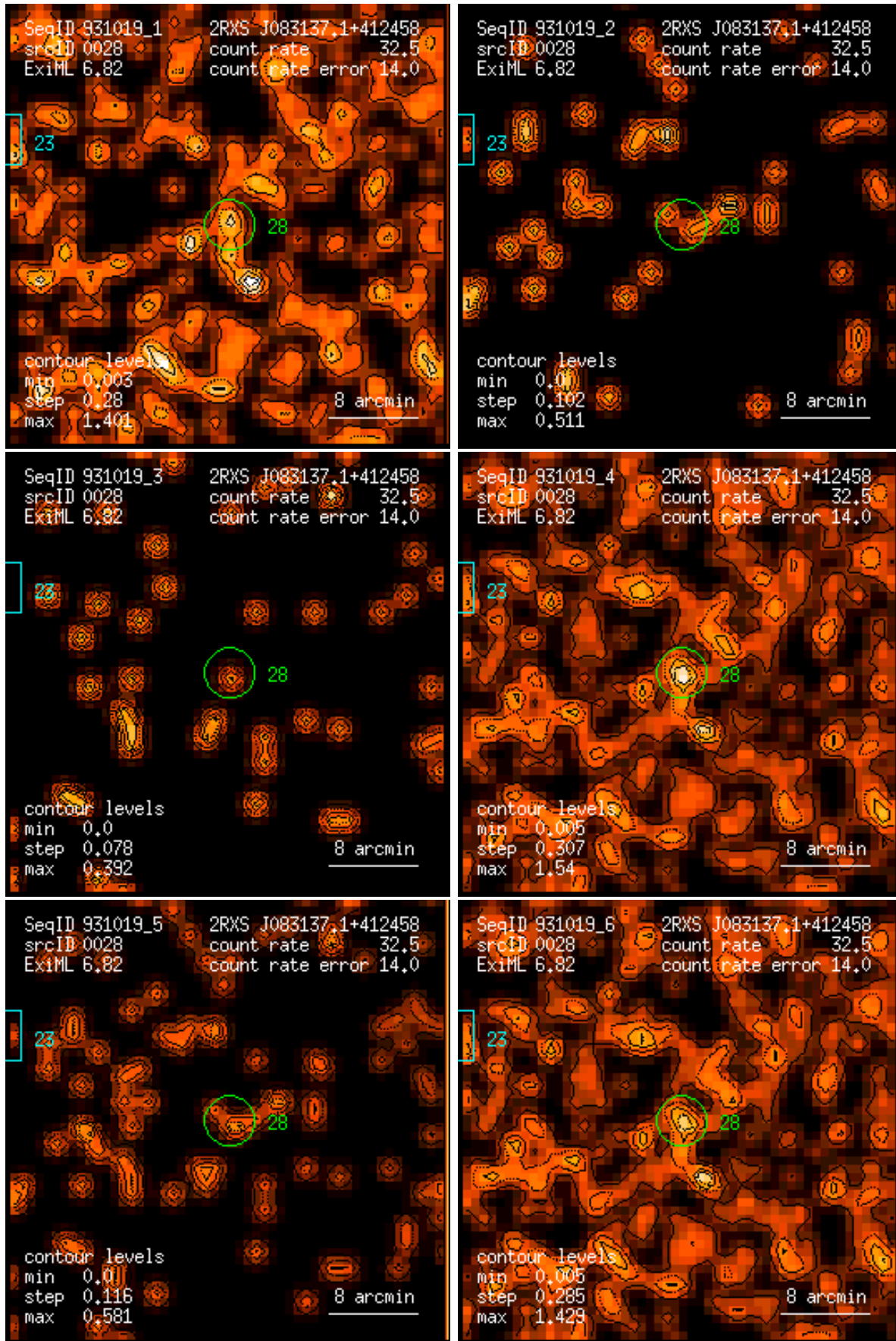
Figure 28: RASS 931019: detection 0028: band rate images, Gaussian filter: (1) PSPC channels 11 – 41, (2) 52 – 90, (3) 91 – 201, (4) 11 – 235, (5) 52 – 201, (6) 11 – 201. Broad band rates in counts/ks. Band rate contour levels in counts/ks/arcmin 2 .
