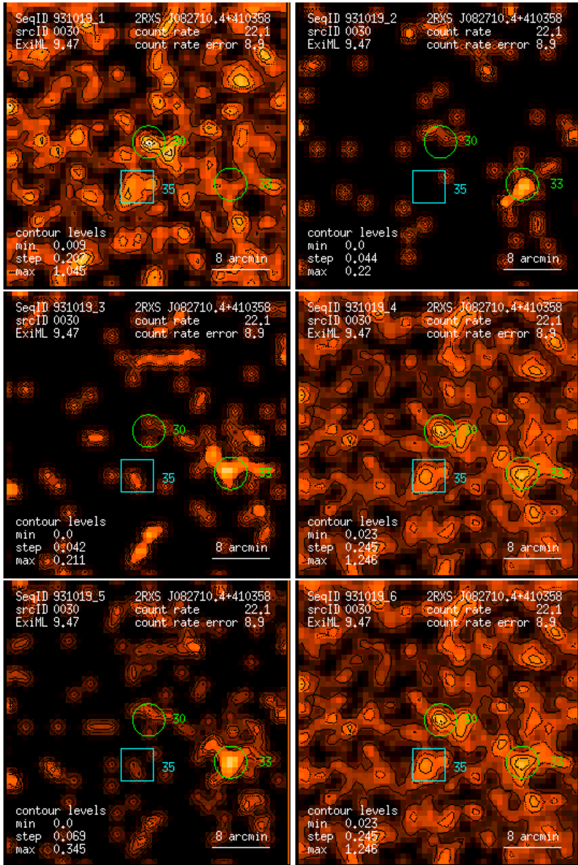
Figure 30: RASS 931019: detection 0030: band rate images, Gaussian filter: (1) PSPC channels 11 – 41, (2) 52 – 90, (3) 91 – 201, (4) 11 – 235, (5) 52 – 201, (6) 11 – 201. Broad band rates in counts/ks. Band rate contour levels in counts/ks/arcmin 2 .
