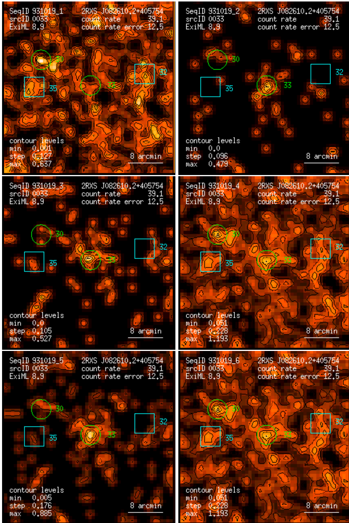
Figure 33: RASS 931019: detection 0033: band rate images, Gaussian filter: (1) PSPC channels 11 – 41, (2) 52 – 90, (3) 91 – 201, (4) 11 – 235, (5) 52 – 201, (6) 11 – 201. Broad band rates in counts/ks. Band rate contour levels in counts/ks/arcmin 2 .
