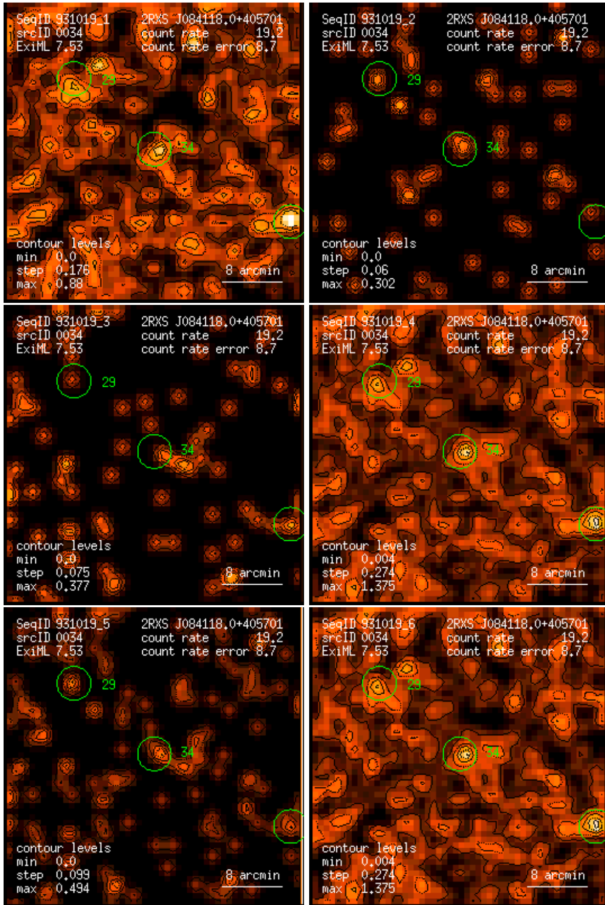
Figure 34: RASS 931019: detection 0034: band rate images, Gaussian filter: (1) PSPC channels 11 – 41, (2) 52 – 90, (3) 91 – 201, (4) 11 – 235, (5) 52 – 201, (6) 11 – 201. Broad band rates in counts/ks. Band rate contour levels in counts/ks/arcmin 2 .
