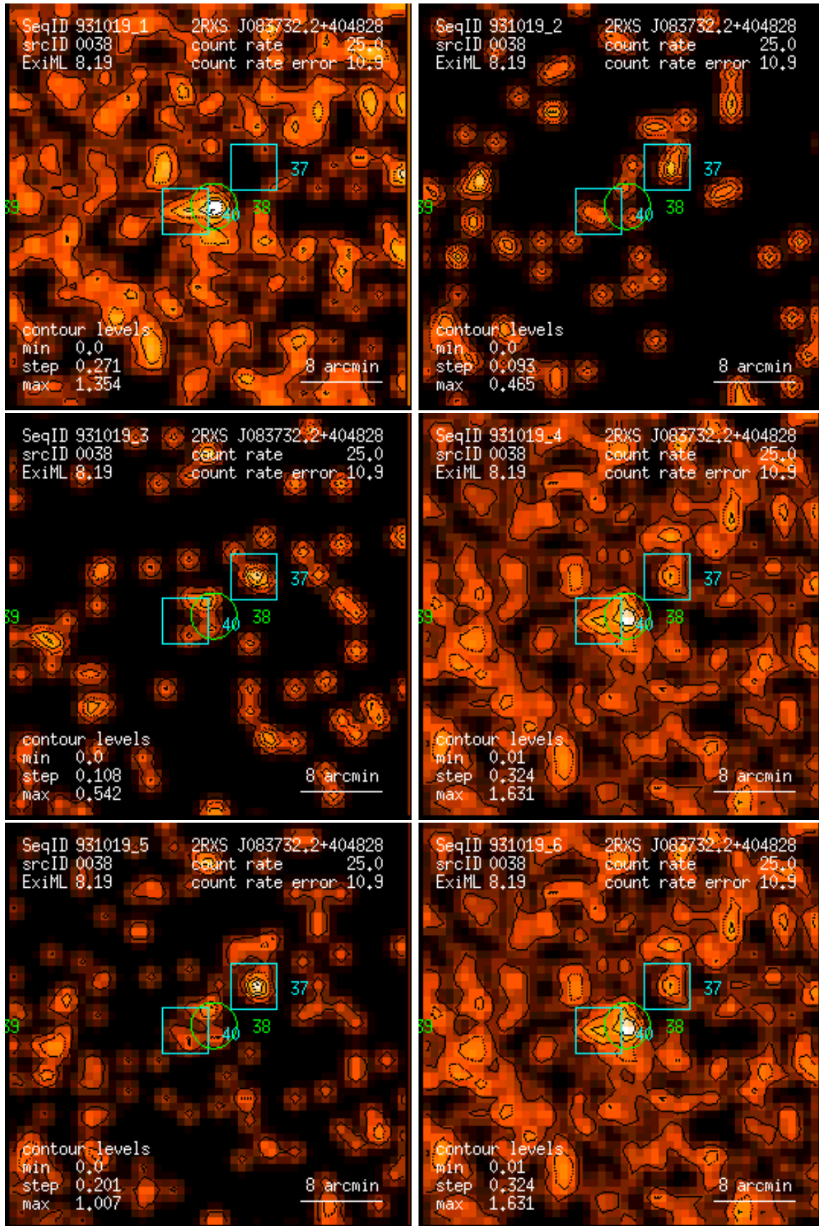
Figure 38: RASS 931019: detection 0038: band rate images, Gaussian filter: (1) PSPC channels 11 – 41, (2) 52 – 90, (3) 91 – 201, (4) 11 – 235, (5) 52 – 201, (6) 11 – 201. Broad band rates in counts/ks. Band rate contour levels in counts/ks/arcmin 2 .
