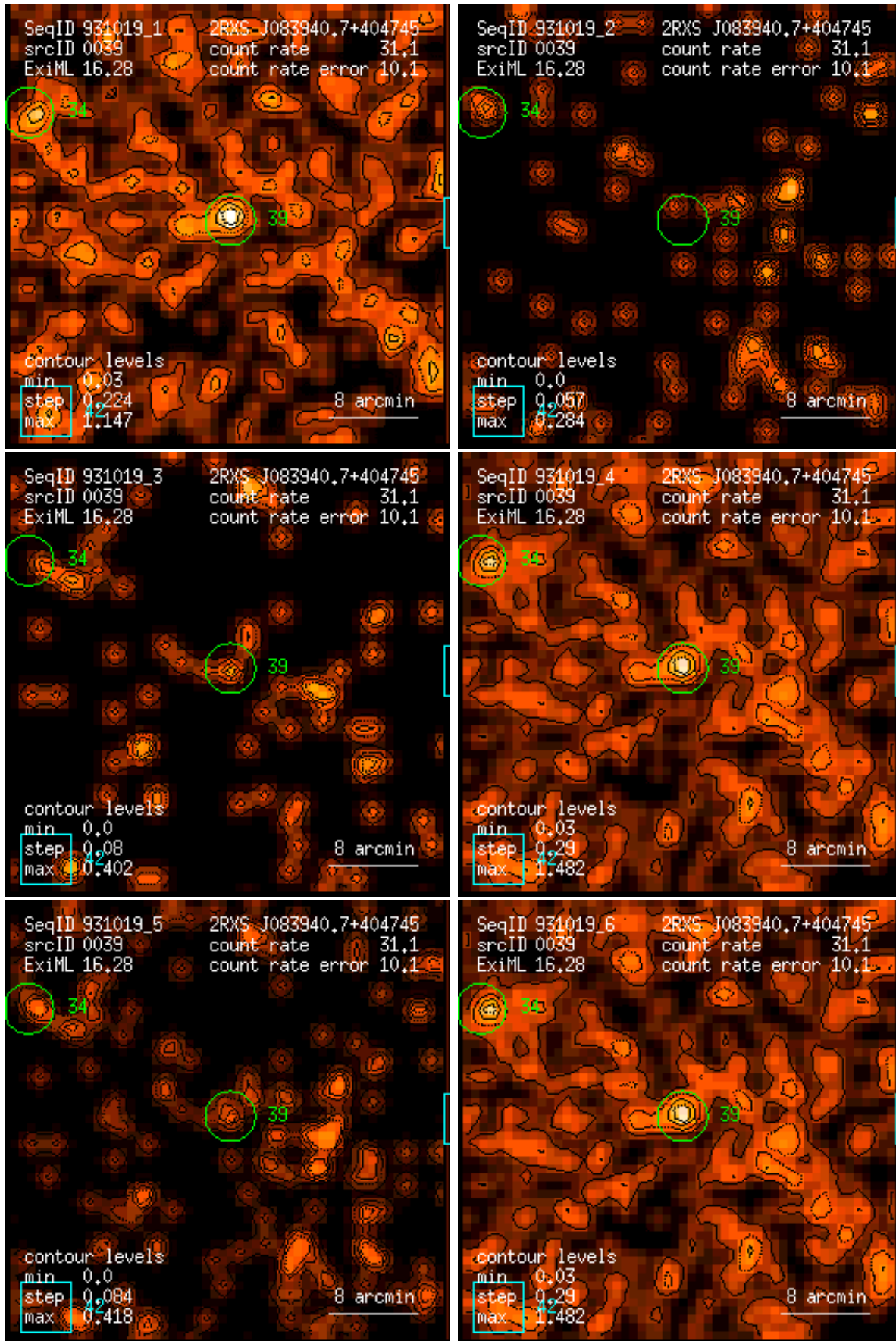
Figure 39: RASS 931019: detection 0039: band rate images, Gaussian filter: (1) PSPC channels 11 – 41, (2) 52 – 90, (3) 91 – 201, (4) 11 – 235, (5) 52 – 201, (6) 11 – 201. Broad band rates in counts/ks. Band rate contour levels in counts/ks/arcmin 2 .
