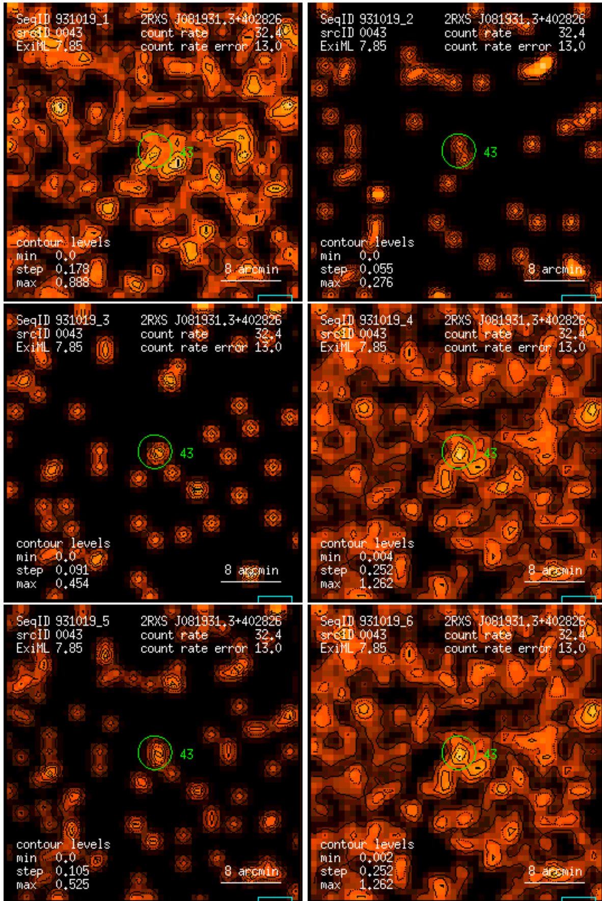
Figure 43: RASS 931019: detection 0043: band rate images, Gaussian filter: (1) PSPC channels 11 – 41, (2) 52 – 90, (3) 91 – 201, (4) 11 – 235, (5) 52 – 201, (6) 11 – 201. Broad band rates in counts/ks. Band rate contour levels in counts/ks/arcmin 2 .
