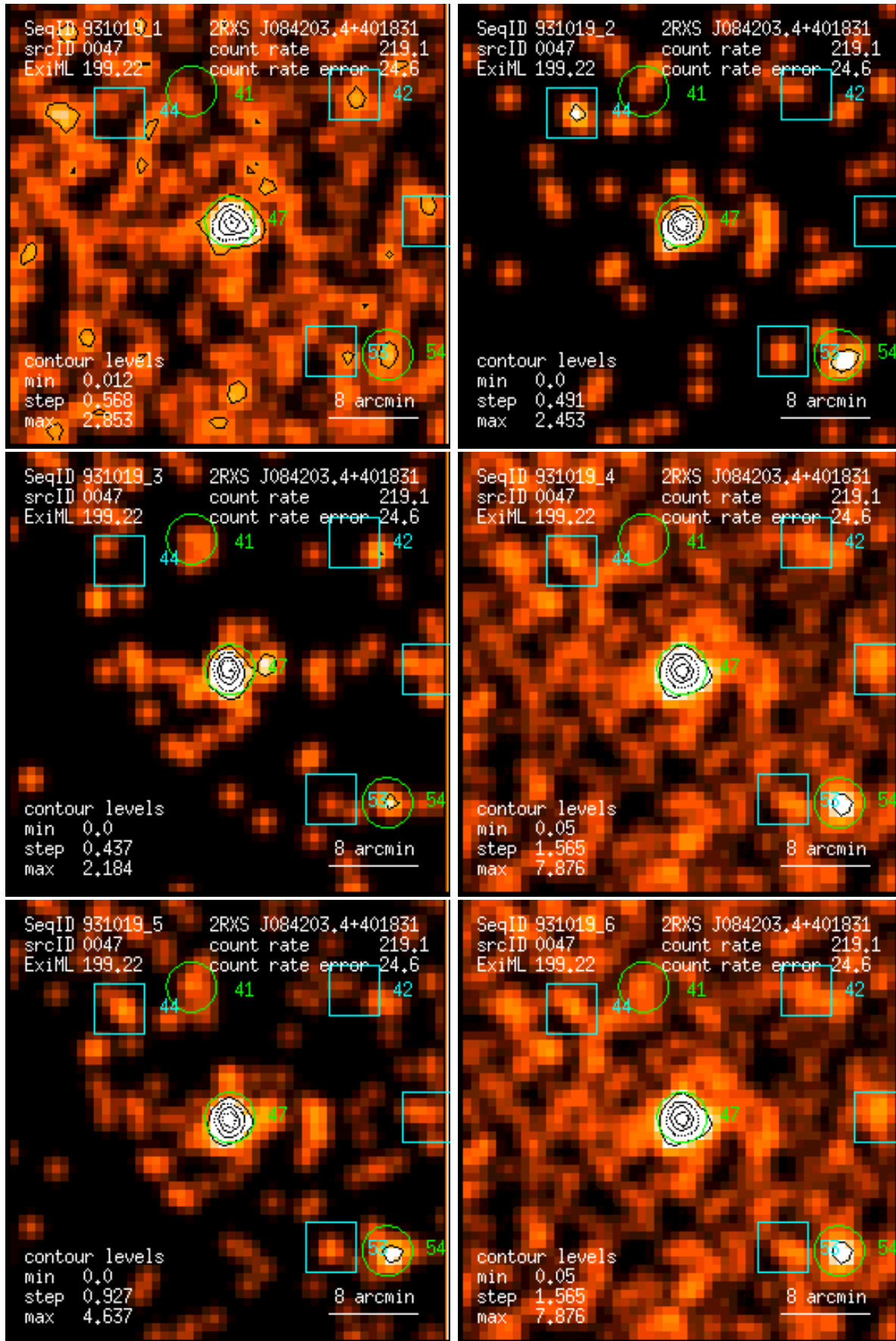
Figure 47: RASS 931019: detection 0047: band rate images, Gaussian filter: (1) PSPC channels 11 – 41, (2) 52 – 90, (3) 91 – 201, (4) 11 – 235, (5) 52 – 201, (6) 11 – 201. Broad band rates in counts/ks. Band rate contour levels in counts/ks/arcmin 2 .
