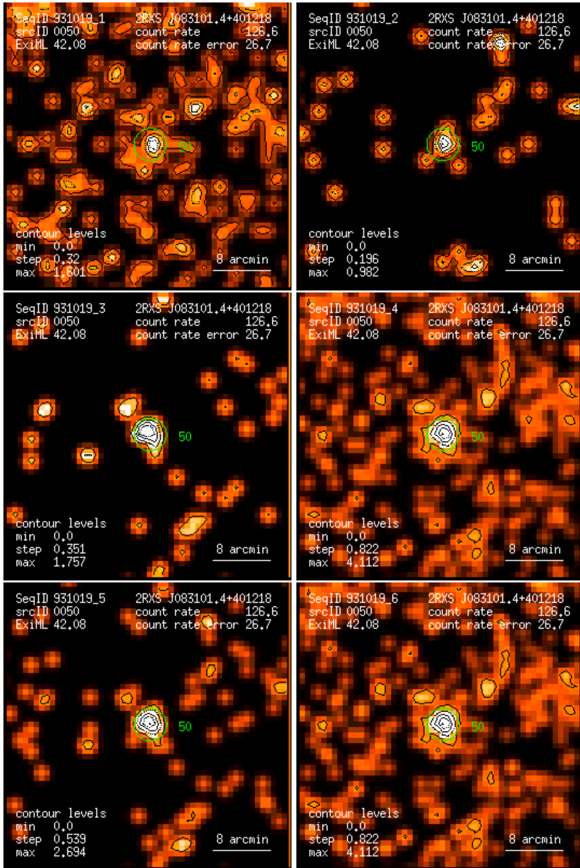
Figure 50: RASS 931019: detection 0050: band rate images, Gaussian filter: (1) PSPC channels 11 – 41, (2) 52 – 90, (3) 91 – 201, (4) 11 – 235, (5) 52 – 201, (6) 11 – 201. Broad band rates in counts/ks. Band rate contour levels in counts/ks/arcmin 2 .
