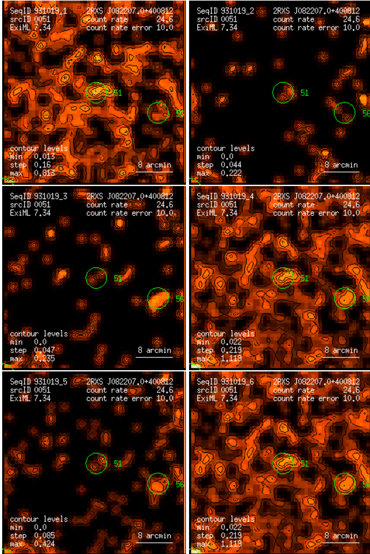
Figure 51: RASS 931019: detection 0051: band rate images, Gaussian filter: (1) PSPC channels 11 – 41, (2) 52 – 90, (3) 91 – 201, (4) 11 – 235, (5) 52 – 201, (6) 11 – 201. Broad band rates in counts/ks. Band rate contour levels in counts/ks/arcmin 2 .
