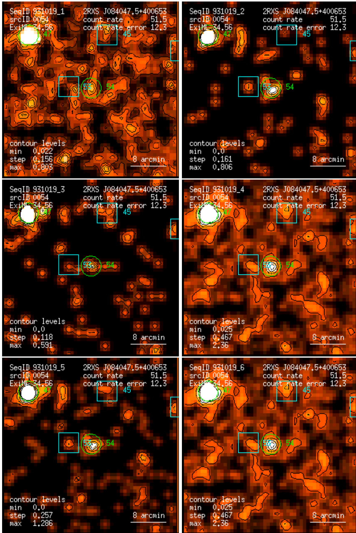
Figure 54: RASS 931019: detection 0054: band rate images, Gaussian filter: (1) PSPC channels 11 – 41, (2) 52 – 90, (3) 91 – 201, (4) 11 – 235, (5) 52 – 201, (6) 11 – 201. Broad band rates in counts/ks. Band rate contour levels in counts/ks/arcmin 2 .
