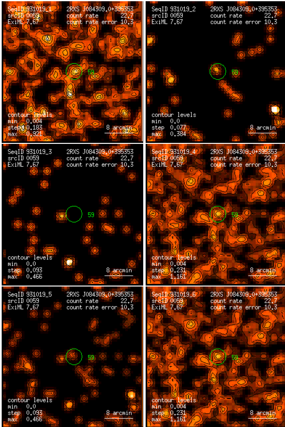
Figure 59: RASS 931019: detection 0059: band rate images, Gaussian filter: (1) PSPC channels 11 – 41, (2) 52 – 90, (3) 91 – 201, (4) 11 – 235, (5) 52 – 201, (6) 11 – 201. Broad band rates in counts/ks. Band rate contour levels in counts/ks/arcmin 2 .
