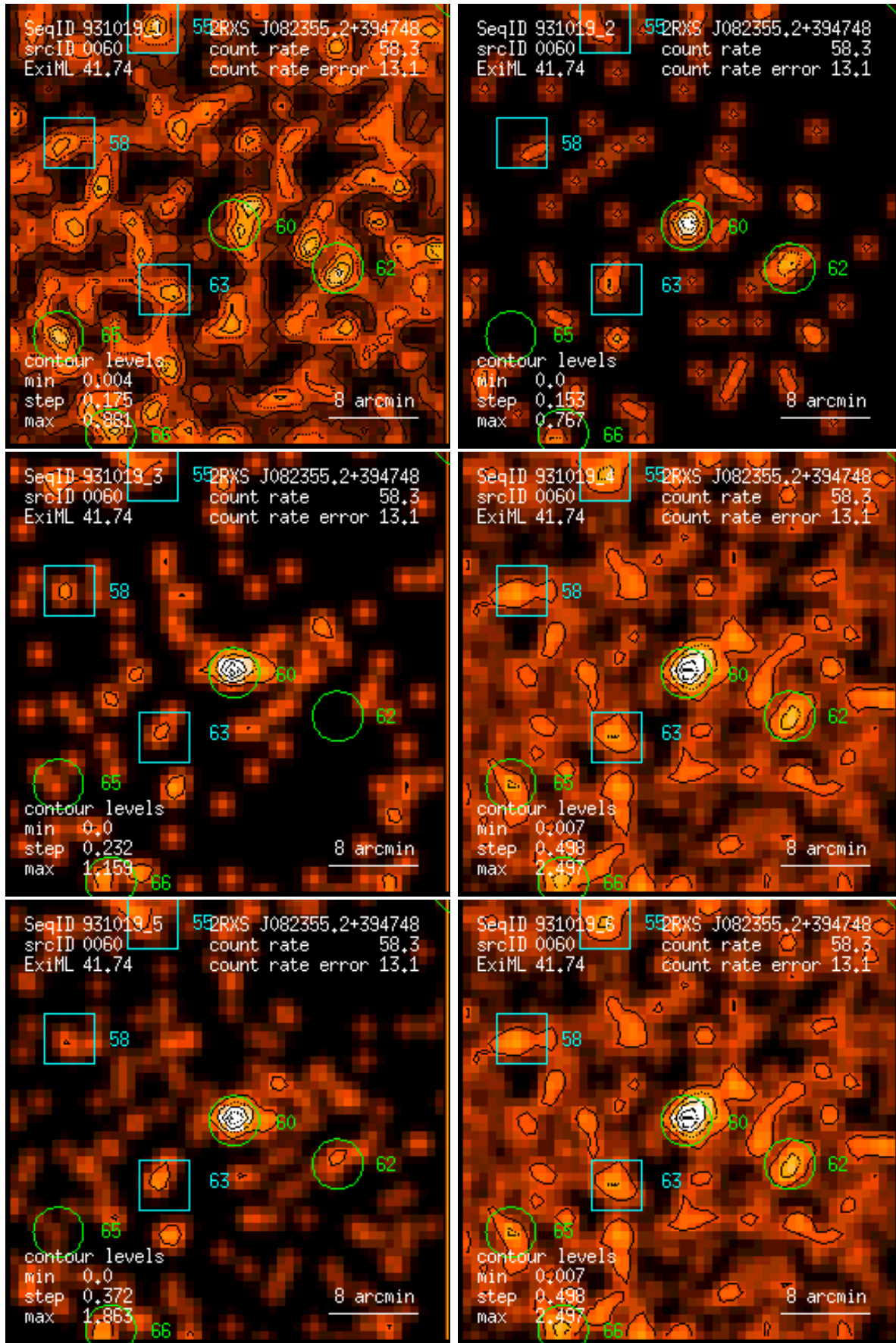
Figure 60: RASS 931019: detection 0060: band rate images, Gaussian filter: (1) PSPC channels 11 – 41, (2) 52 – 90, (3) 91 – 201, (4) 11 – 235, (5) 52 – 201, (6) 11 – 201. Broad band rates in counts/ks. Band rate contour levels in counts/ks/arcmin 2 .
