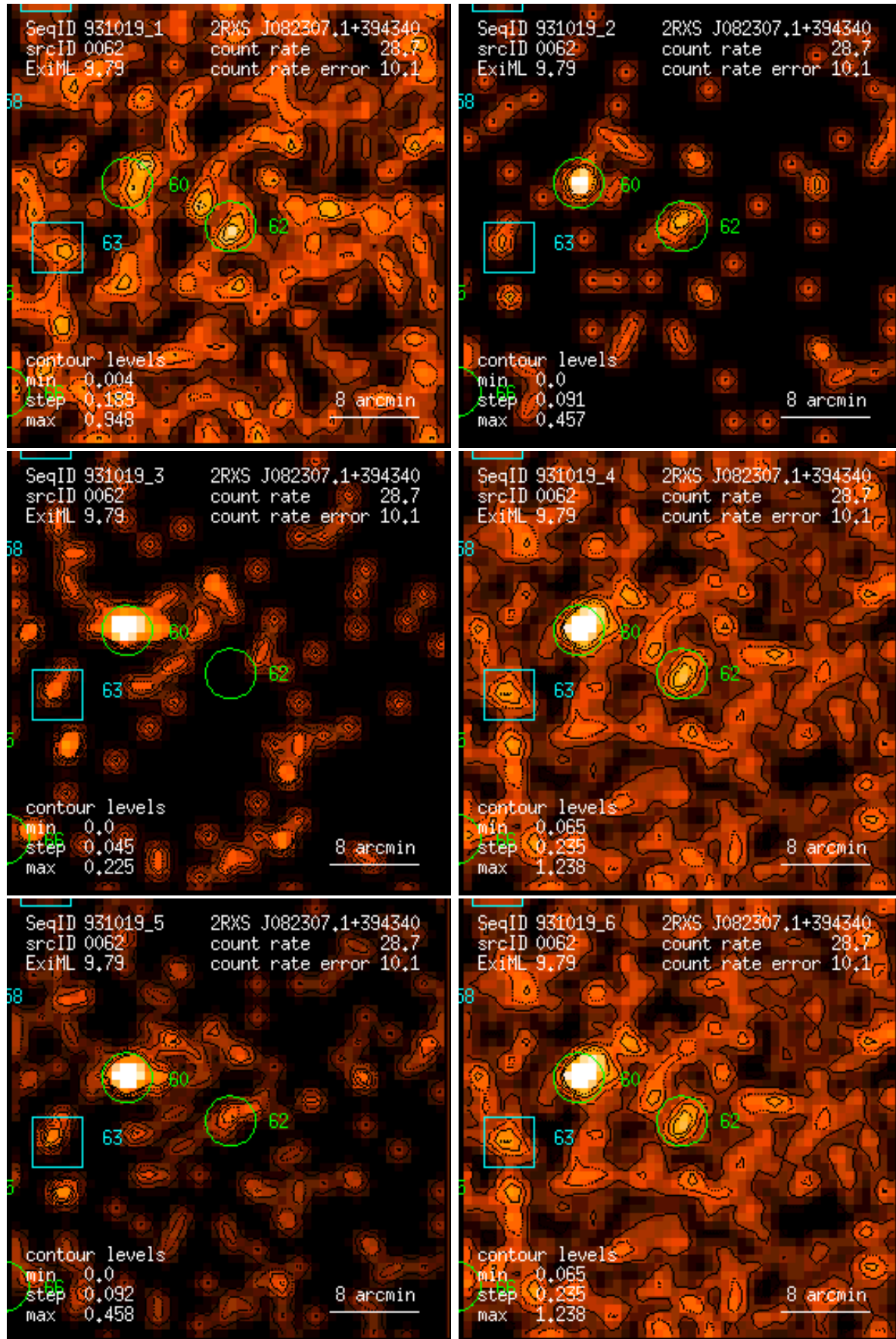
Figure 62: RASS 931019: detection 0062: band rate images, Gaussian filter: (1) PSPC channels 11 – 41, (2) 52 – 90, (3) 91 – 201, (4) 11 – 235, (5) 52 – 201, (6) 11 – 201. Broad band rates in counts/ks. Band rate contour levels in counts/ks/arcmin 2 .
