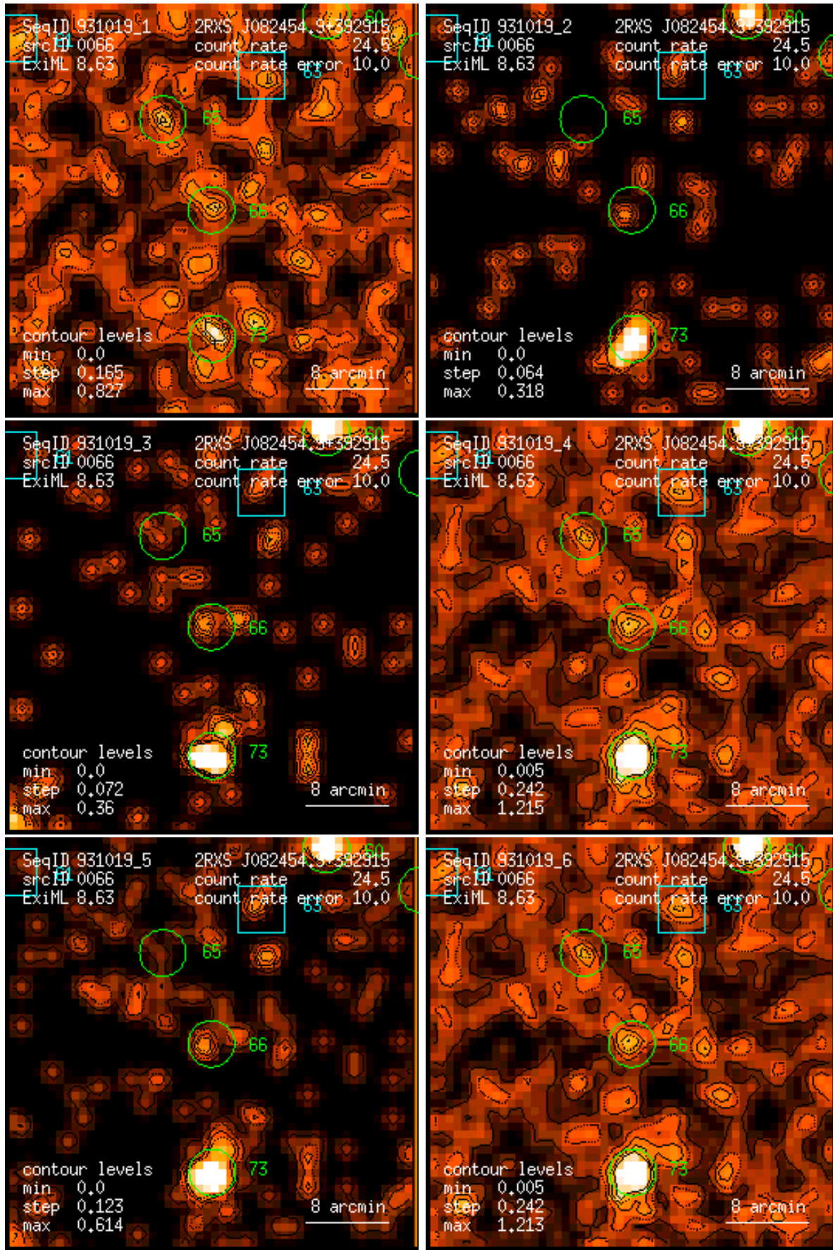
Figure 66: RASS 931019: detection 0066: band rate images, Gaussian filter: (1) PSPC channels 11 – 41, (2) 52 – 90, (3) 91 – 201, (4) 11 – 235, (5) 52 – 201, (6) 11 – 201. Broad band rates in counts/ks. Band rate contour levels in counts/ks/arcmin 2 .
