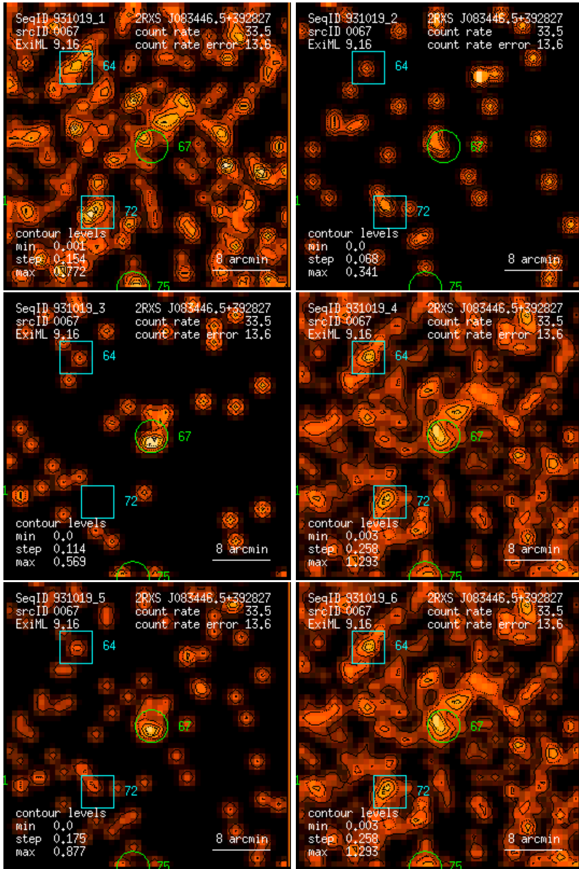
Figure 67: RASS 931019: detection 0067: band rate images, Gaussian filter: (1) PSPC channels 11 – 41, (2) 52 – 90, (3) 91 – 201, (4) 11 – 235, (5) 52 – 201, (6) 11 – 201. Broad band rates in counts/ks. Band rate contour levels in counts/ks/arcmin 2 .
