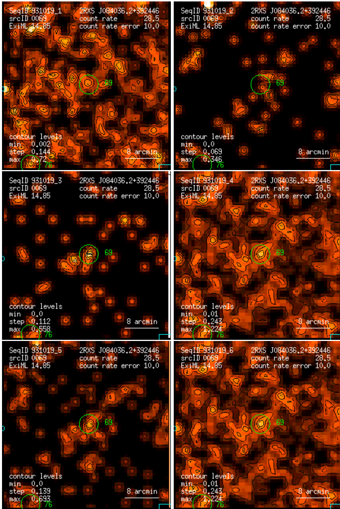
Figure 69: RASS 931019: detection 0069: band rate images, Gaussian filter: (1) PSPC channels 11 – 41, (2) 52 – 90, (3) 91 – 201, (4) 11 – 235, (5) 52 – 201, (6) 11 – 201. Broad band rates in counts/ks. Band rate contour levels in counts/ks/arcmin 2 .
