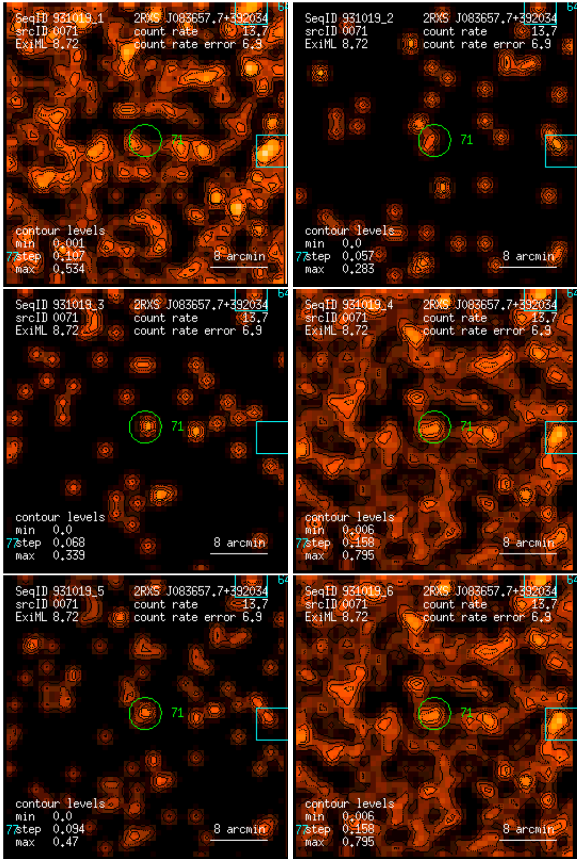
Figure 71: RASS 931019: detection 0071: band rate images, Gaussian filter: (1) PSPC channels 11 – 41, (2) 52 – 90, (3) 91 – 201, (4) 11 – 235, (5) 52 – 201, (6) 11 – 201. Broad band rates in counts/ks. Band rate contour levels in counts/ks/arcmin 2 .
