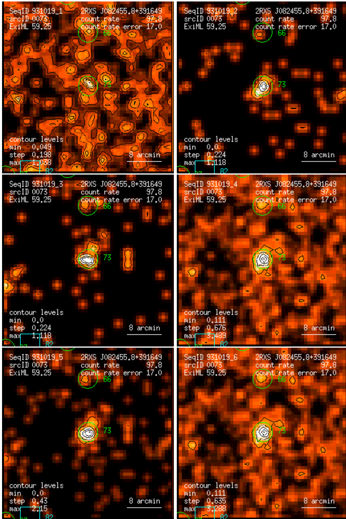
Figure 73: RASS 931019: detection 0073: band rate images, Gaussian filter: (1) PSPC channels 11 – 41, (2) 52 – 90, (3) 91 – 201, (4) 11 – 235, (5) 52 – 201, (6) 11 – 201. Broad band rates in counts/ks. Band rate contour levels in counts/ks/arcmin 2 .
