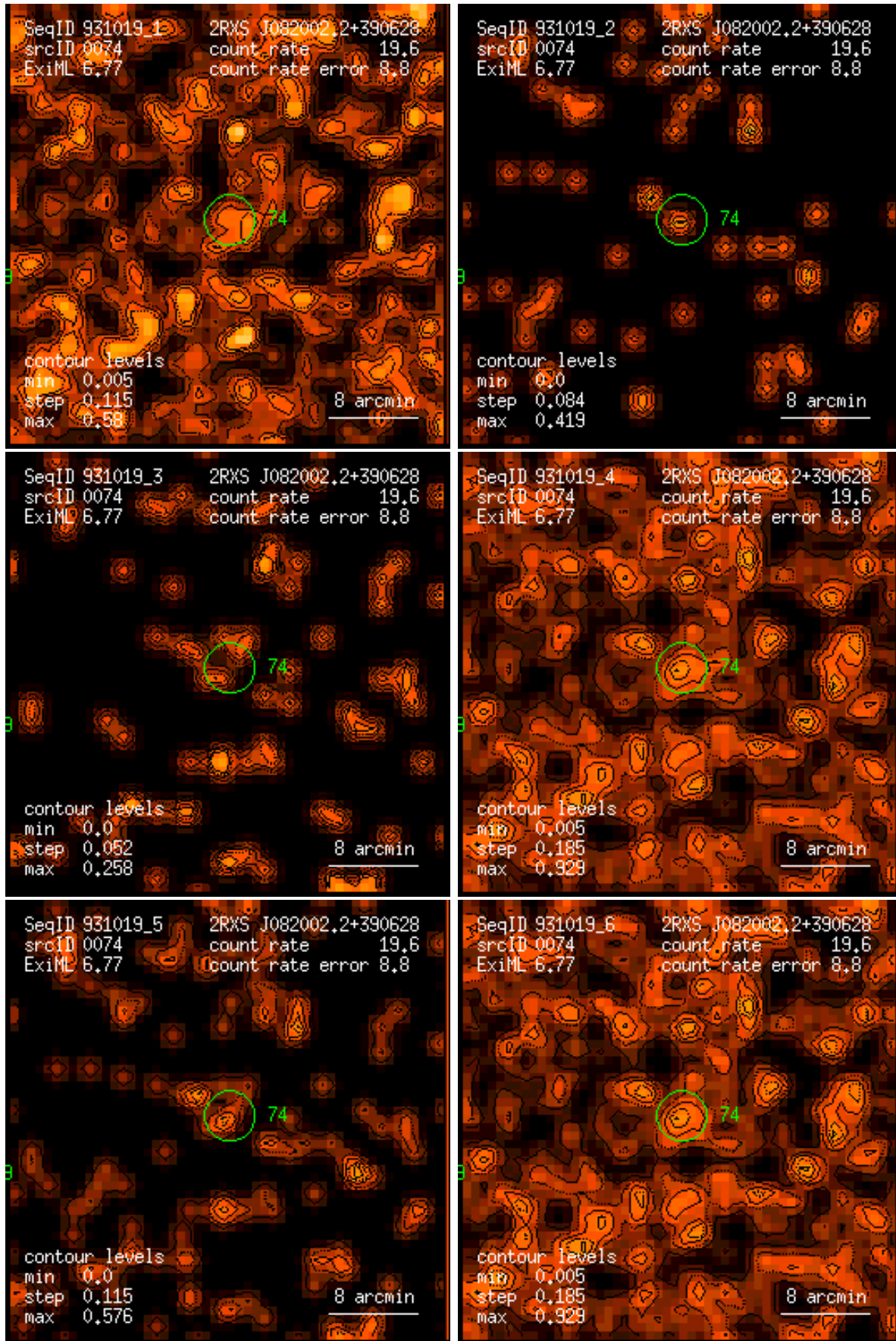
Figure 74: RASS 931019: detection 0074: band rate images, Gaussian filter: (1) PSPC channels 11 – 41, (2) 52 – 90, (3) 91 – 201, (4) 11 – 235, (5) 52 – 201, (6) 11 – 201. Broad band rates in counts/ks. Band rate contour levels in counts/ks/arcmin 2 .
