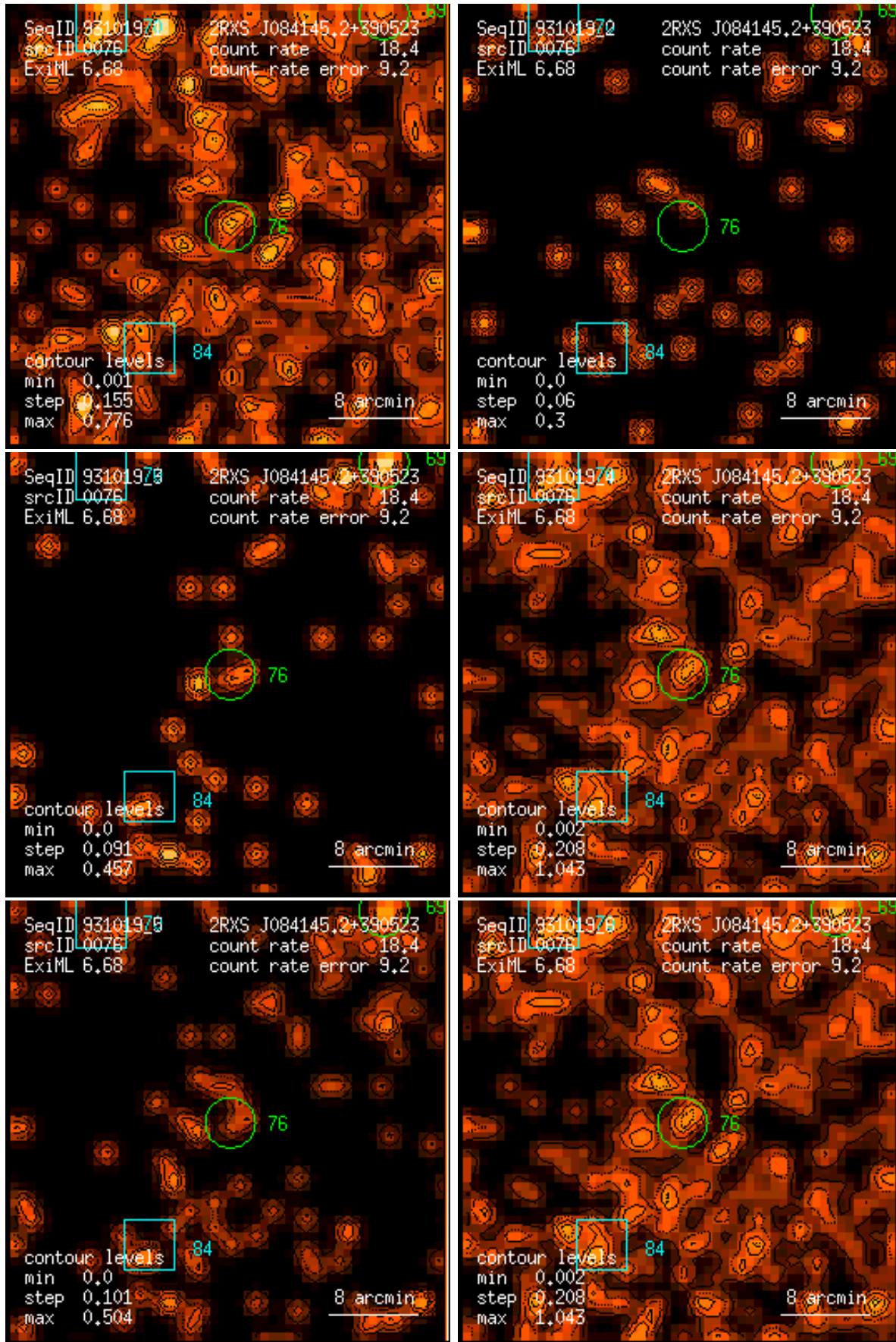
Figure 76: RASS 931019: detection 0076: band rate images, Gaussian filter: (1) PSPC channels 11 – 41, (2) 52 – 90, (3) 91 – 201, (4) 11 – 235, (5) 52 – 201, (6) 11 – 201. Broad band rates in counts/ks. Band rate contour levels in counts/ks/arcmin 2 .
