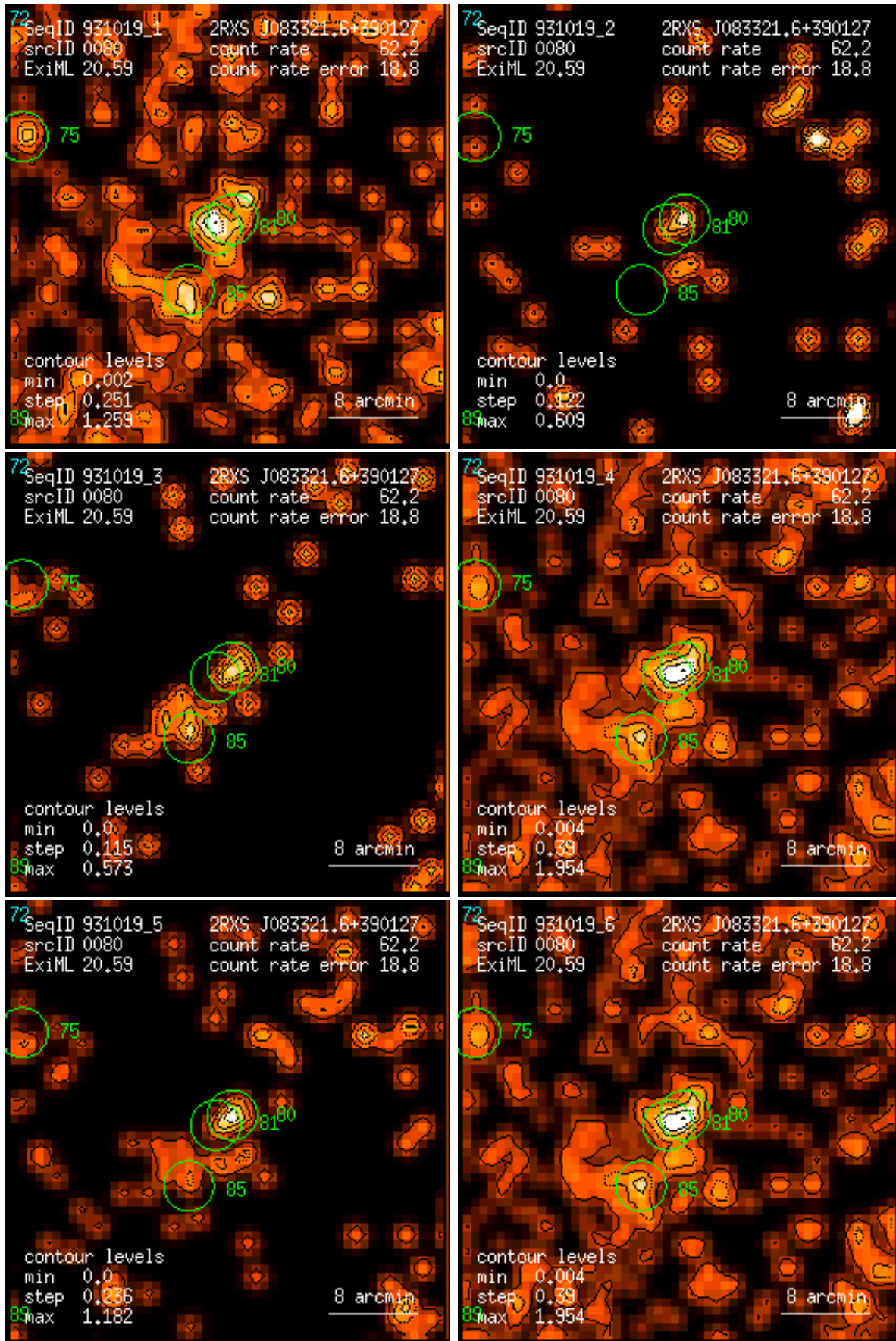
Figure 80: RASS 931019: detection 0080: band rate images, Gaussian filter: (1) PSPC channels 11 – 41, (2) 52 – 90, (3) 91 – 201, (4) 11 – 235, (5) 52 – 201, (6) 11 – 201. Broad band rates in counts/ks. Band rate contour levels in counts/ks/arcmin 2 .
