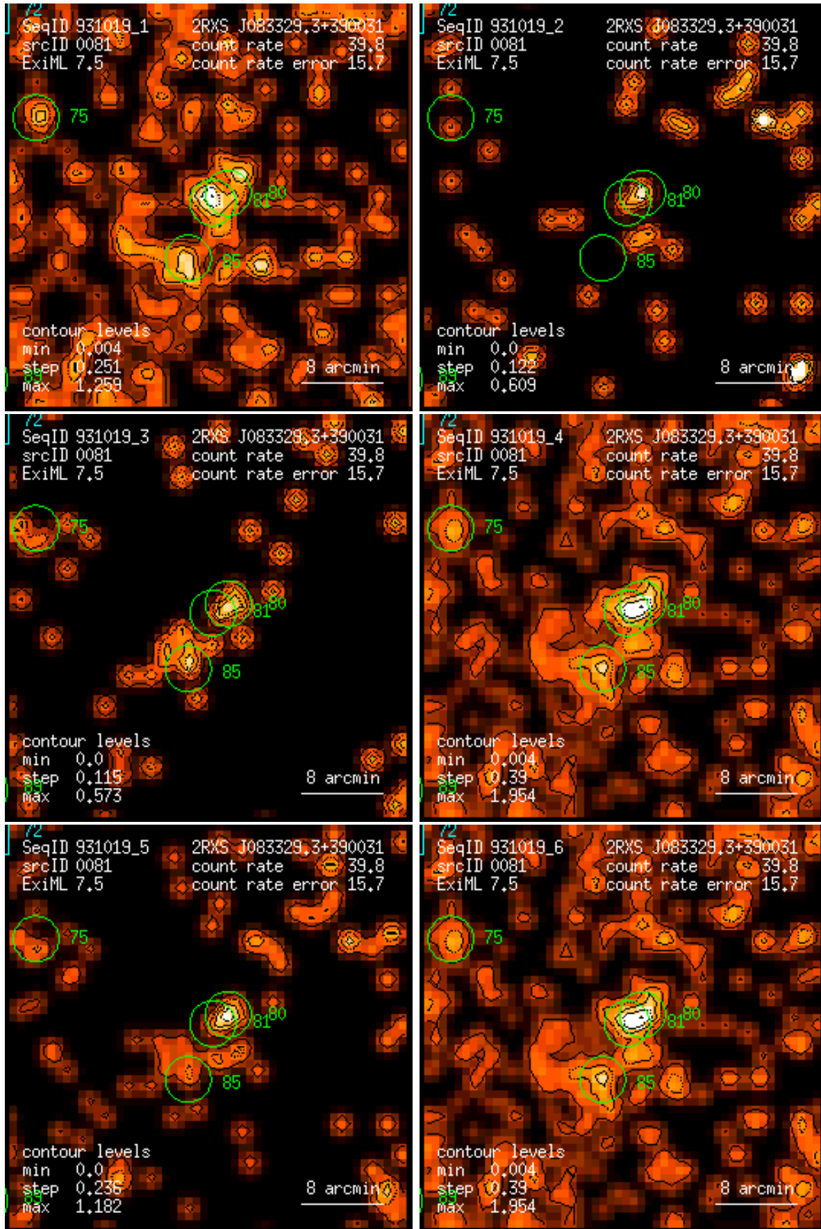
Figure 81: RASS 931019: detection 0081: band rate images, Gaussian filter: (1) PSPC channels 11 – 41, (2) 52 – 90, (3) 91 – 201, (4) 11 – 235, (5) 52 – 201, (6) 11 – 201. Broad band rates in counts/ks. Band rate contour levels in counts/ks/arcmin 2 .
