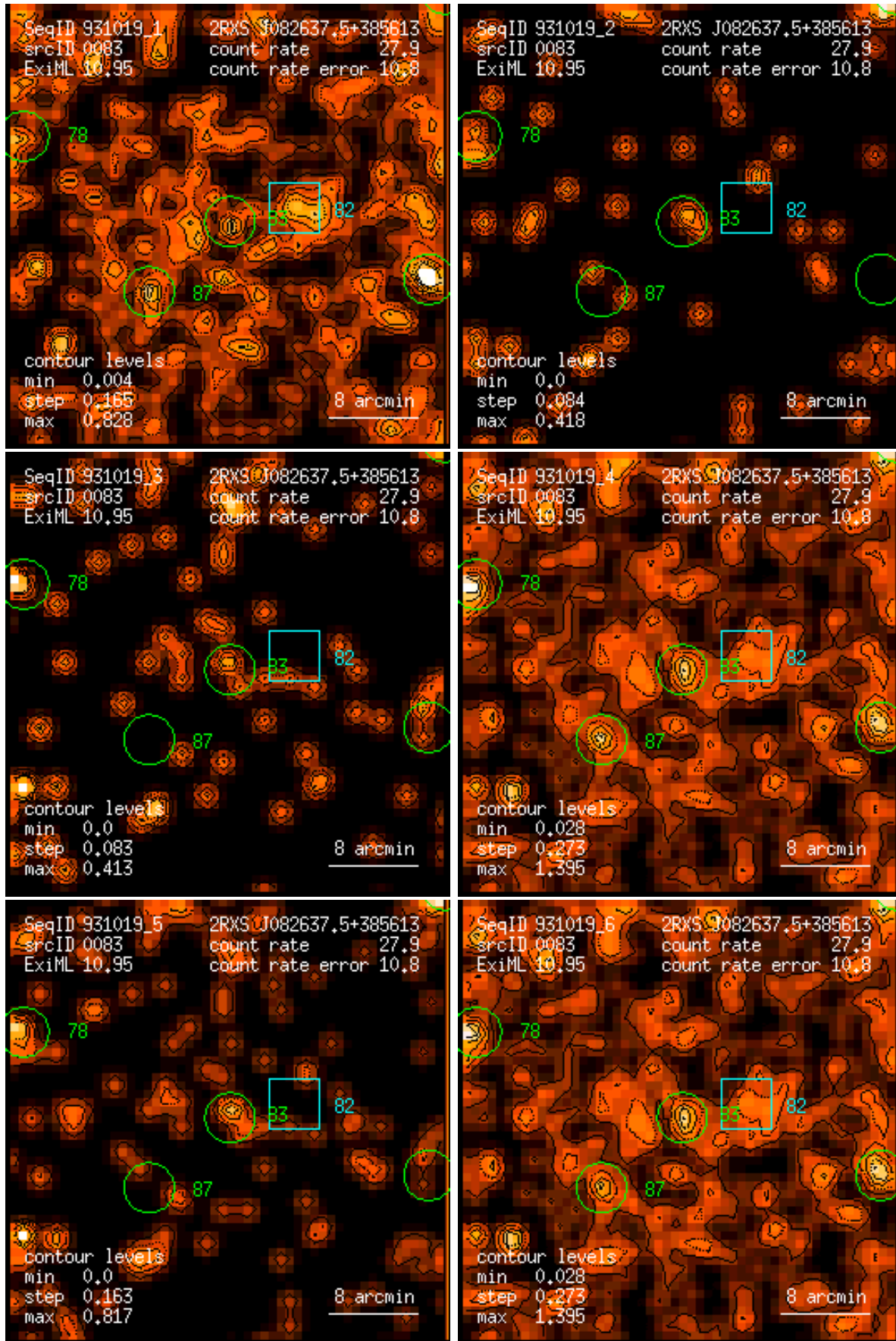
Figure 83: RASS 931019: detection 0083: band rate images, Gaussian filter: (1) PSPC channels 11 – 41, (2) 52 – 90, (3) 91 – 201, (4) 11 – 235, (5) 52 – 201, (6) 11 – 201. Broad band rates in counts/ks. Band rate contour levels in counts/ks/arcmin 2 .
