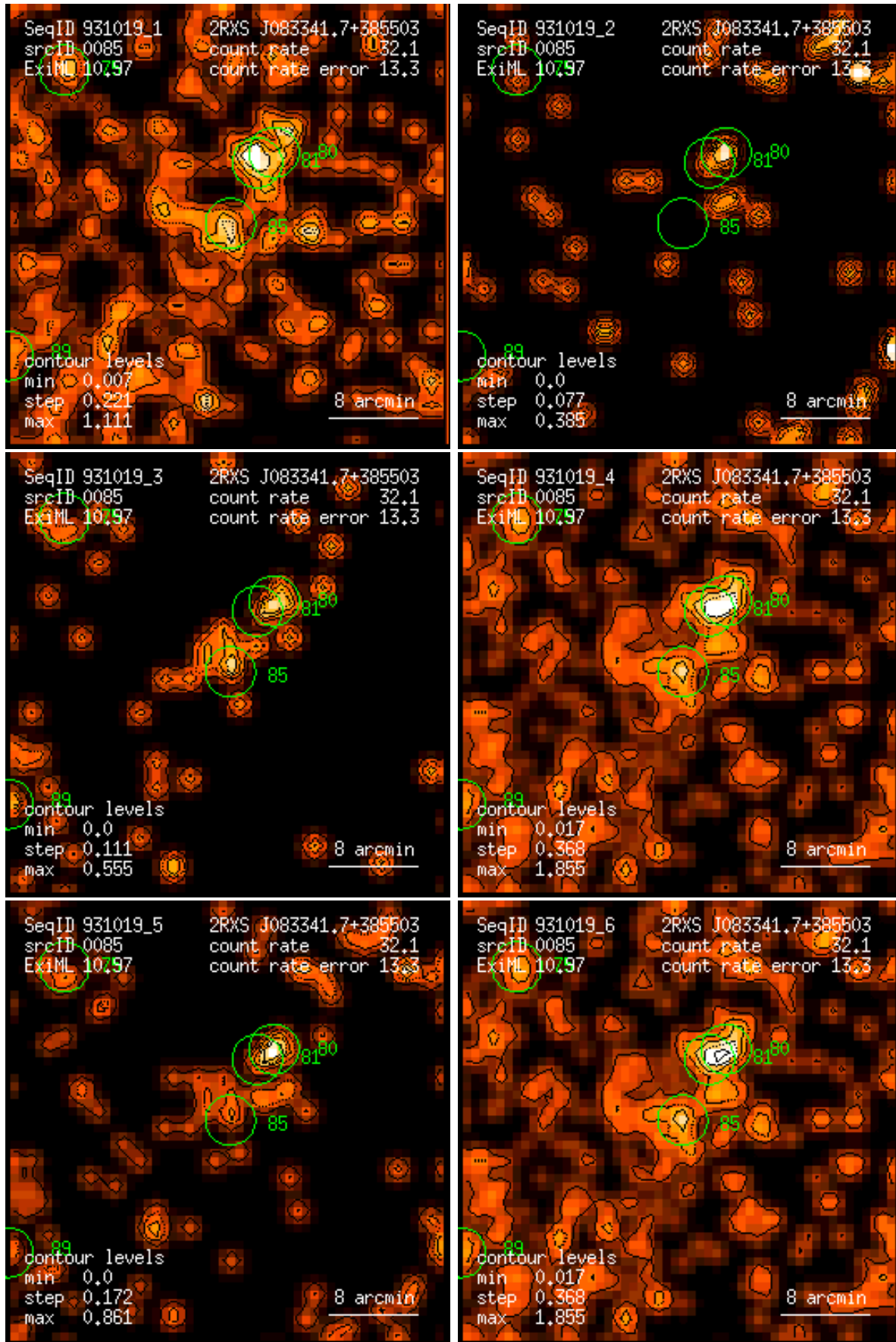
Figure 85: RASS 931019: detection 0085: band rate images, Gaussian filter: (1) PSPC channels 11 – 41, (2) 52 – 90, (3) 91 – 201, (4) 11 – 235, (5) 52 – 201, (6) 11 – 201. Broad band rates in counts/ks. Band rate contour levels in counts/ks/arcmin 2 .
