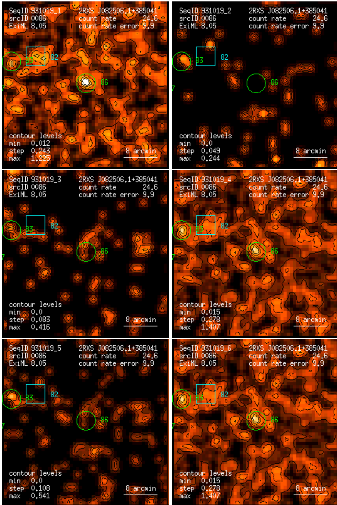
Figure 86: RASS 931019: detection 0086: band rate images, Gaussian filter: (1) PSPC channels 11 – 41, (2) 52 – 90, (3) 91 – 201, (4) 11 – 235, (5) 52 – 201, (6) 11 – 201. Broad band rates in counts/ks. Band rate contour levels in counts/ks/arcmin 2 .
