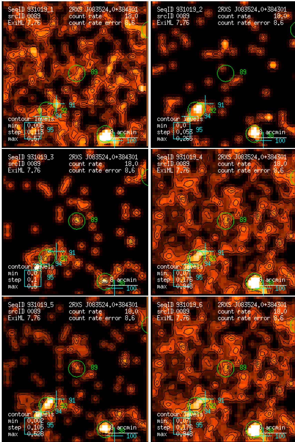
Figure 89: RASS 931019: detection 0089: band rate images, Gaussian filter: (1) PSPC channels 11 – 41, (2) 52 – 90, (3) 91 – 201, (4) 11 – 235, (5) 52 – 201, (6) 11 – 201. Broad band rates in counts/ks. Band rate contour levels in counts/ks/arcmin 2 .
