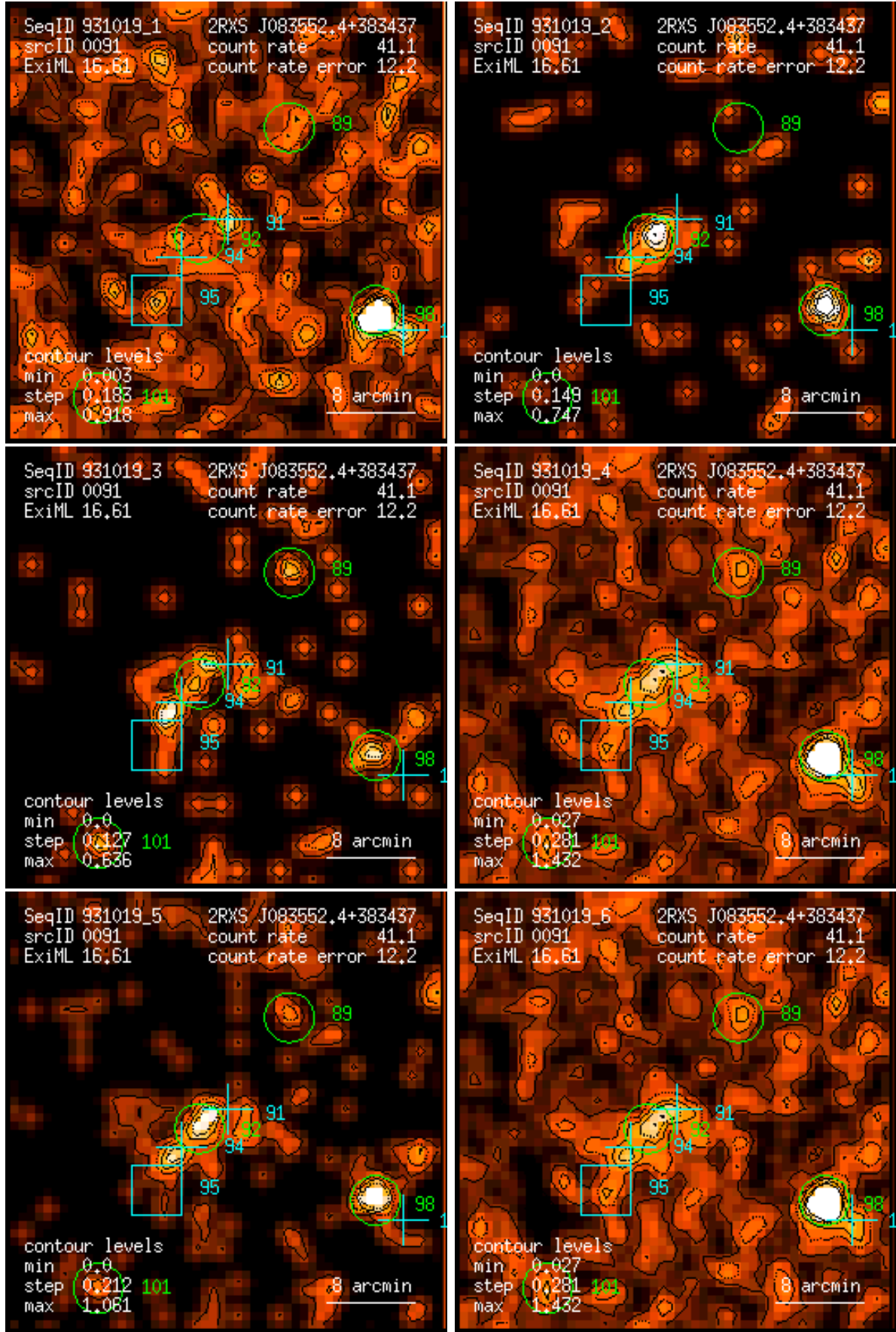
Figure 91: RASS 931019: detection 0091: band rate images, Gaussian filter: (1) PSPC channels 11 – 41, (2) 52 – 90, (3) 91 – 201, (4) 11 – 235, (5) 52 – 201, (6) 11 – 201. Broad band rates in counts/ks. Band rate contour levels in counts/ks/arcmin 2 .
