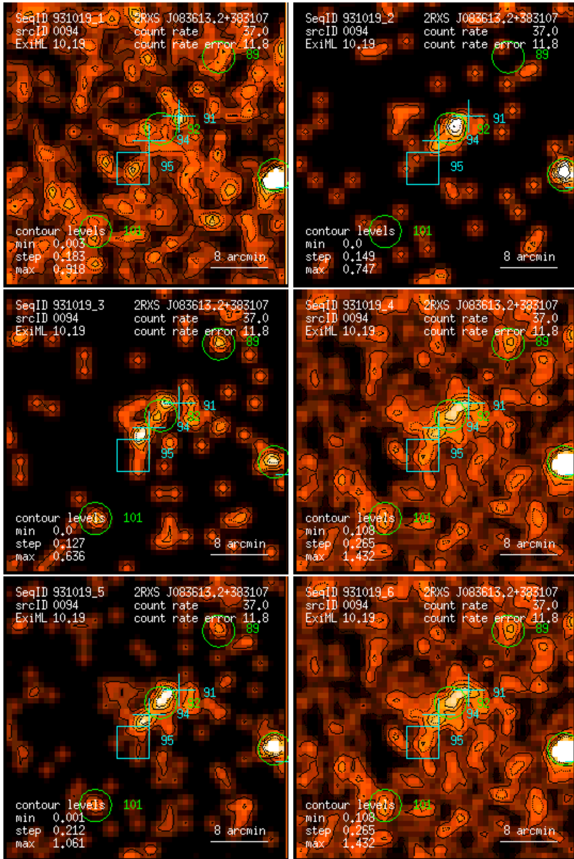
Figure 94: RASS 931019: detection 0094: band rate images, Gaussian filter: (1) PSPC channels 11 – 41, (2) 52 – 90, (3) 91 – 201, (4) 11 – 235, (5) 52 – 201, (6) 11 – 201. Broad band rates in counts/ks. Band rate contour levels in counts/ks/arcmin 2 .
