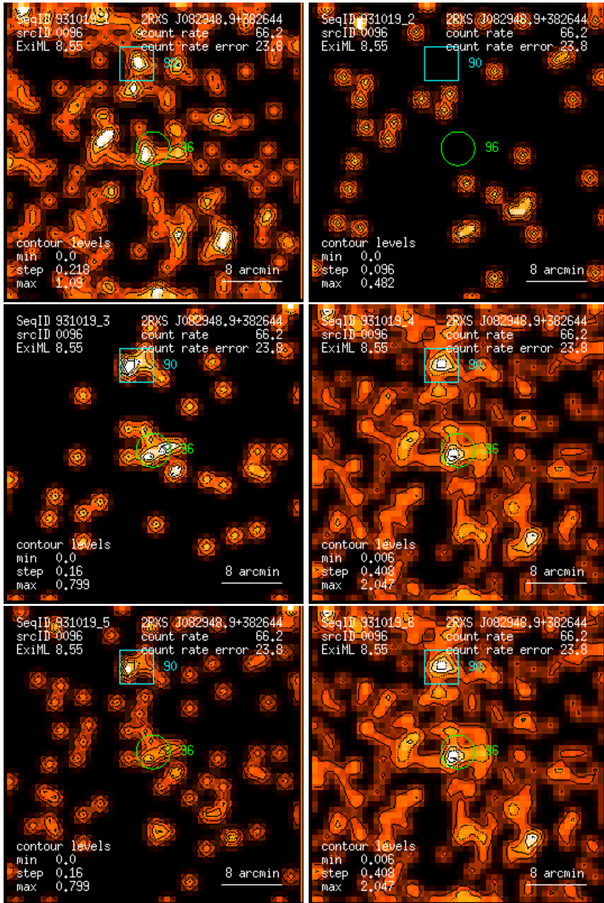
Figure 96: RASS 931019: detection 0096: band rate images, Gaussian filter: (1) PSPC channels 11 – 41, (2) 52 – 90, (3) 91 – 201, (4) 11 – 235, (5) 52 – 201, (6) 11 – 201. Broad band rates in counts/ks. Band rate contour levels in counts/ks/arcmin 2 .
